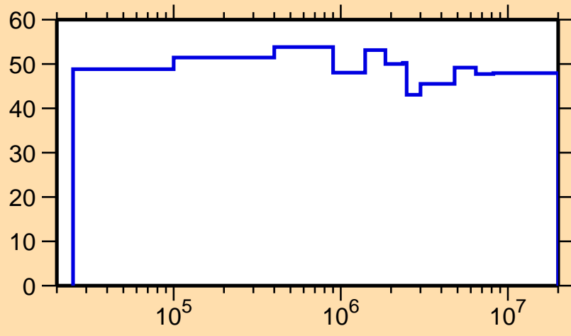
\Delta\sigma/\sigma vs. E for ^{177}\text{W}(n,n_1)
