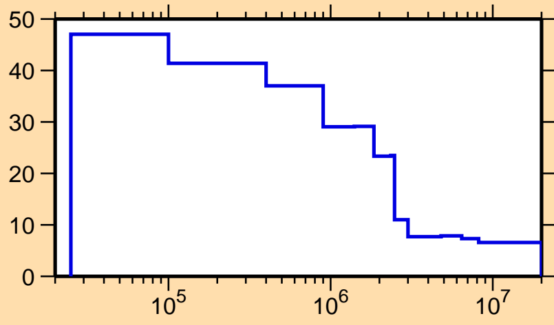
\Delta\sigma/\sigma vs. E for ^{177}\text{W}(n,\text{nonel.})
