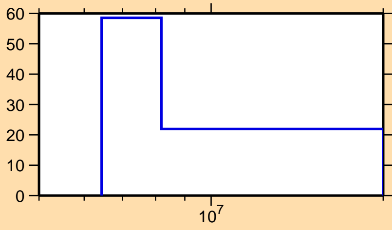
\Delta\sigma/\sigma vs. E for ^{177}\text{W}(n,2n)
