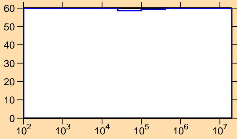
\Delta\sigma/\sigma vs. E for ^{177}\text{W}(n,\gamma)
