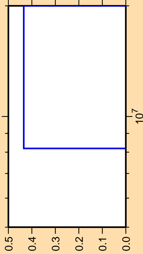
\Delta\sigma/\sigma vs. E for ^{177}\text{W}(n,3n\alpha)
