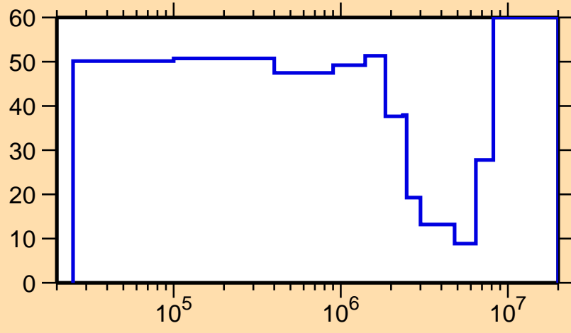
\Delta\sigma/\sigma vs. E for ^{177}\text{W}(n,\text{inel.})
