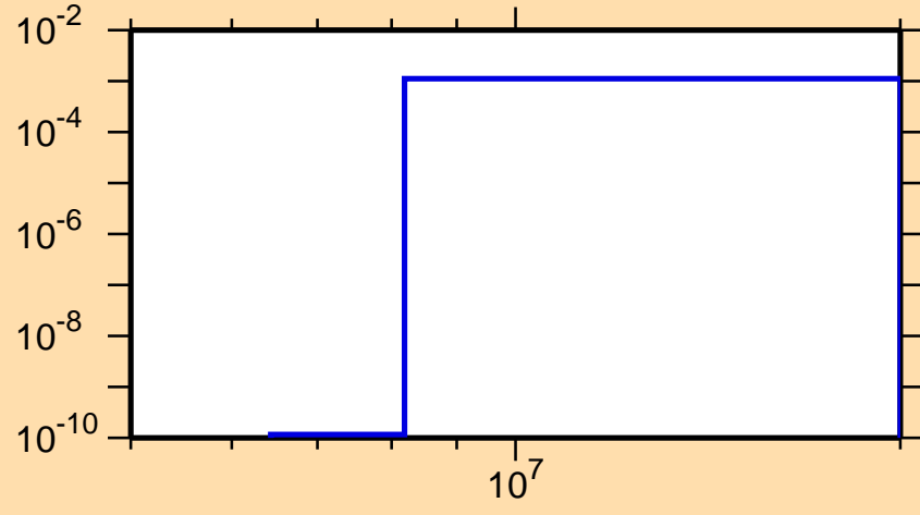
\sigma vs. E for ^{177}\text{W}(n,d)
