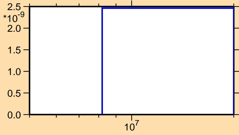
\sigma vs. E for ^{178}\text{W}(n,2np)
