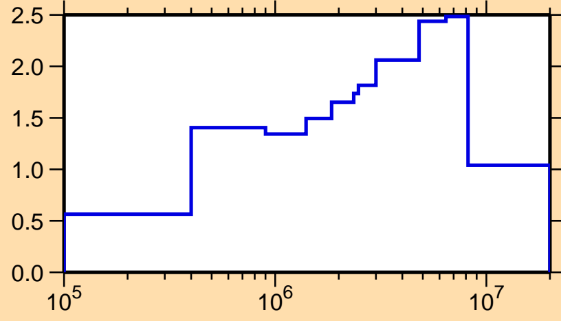
\sigma vs. E for ^{178}\text{W}(n,\text{inel.})
