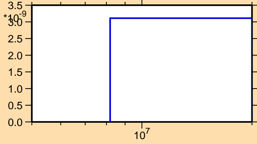
\sigma vs. E for ^{178}\text{W}(n,p\alpha)
