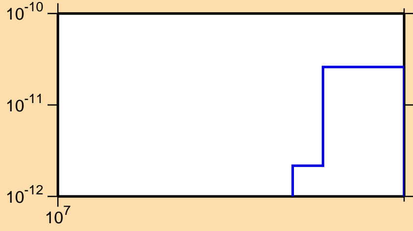
\sigma vs. E for ^{179}\text{W} (mt 45)
