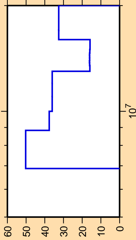
\Delta\sigma/\sigma vs. E for ^{179}\text{W}(n,2n)
