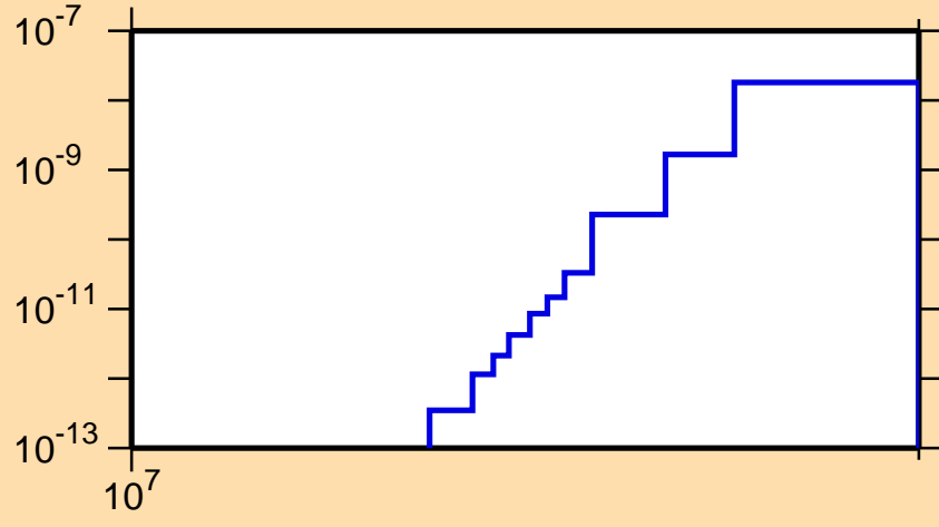
\sigma vs. E for ^{179}\text{W}(n,\text{He3})
