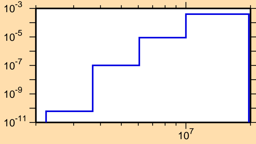
\sigma vs. E for ^{179}\text{W}(n,n\alpha)
