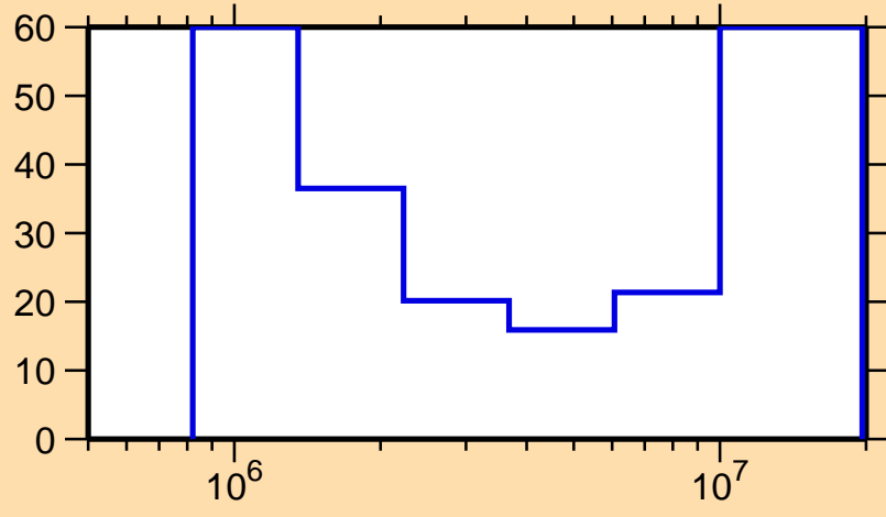
\Delta\sigma/\sigma vs. E for ^{179}\text{W}(n,n\text{cont.})
