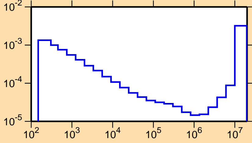
\sigma vs. E for ^{179}\text{W}(n,\alpha)
