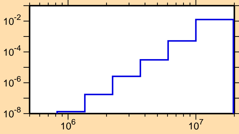
\sigma vs. E for ^{179}\text{W}(n,p)
