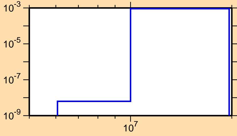
\sigma vs. E for ^{179}\text{W}(n,np)
