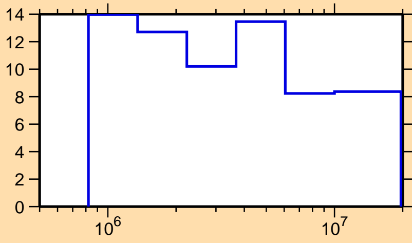
\Delta\sigma/\sigma vs. E for ^{179}\text{W}(n, el.)
