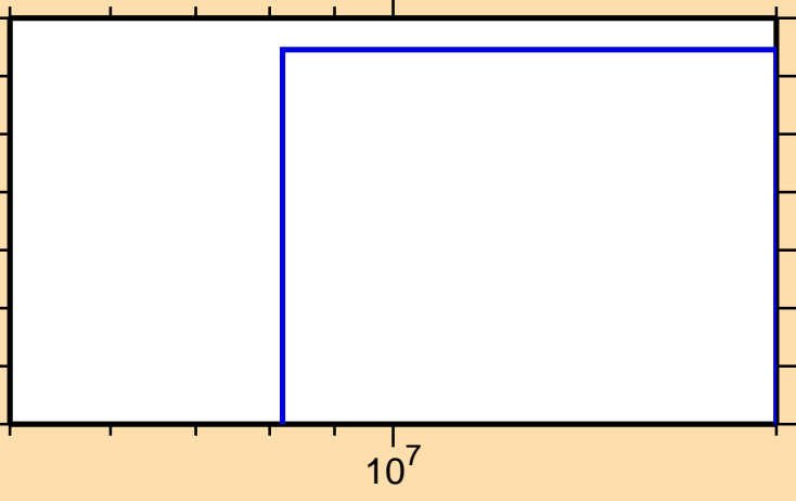
\sigma vs. E for ^{179}\text{W} (mt 45)
