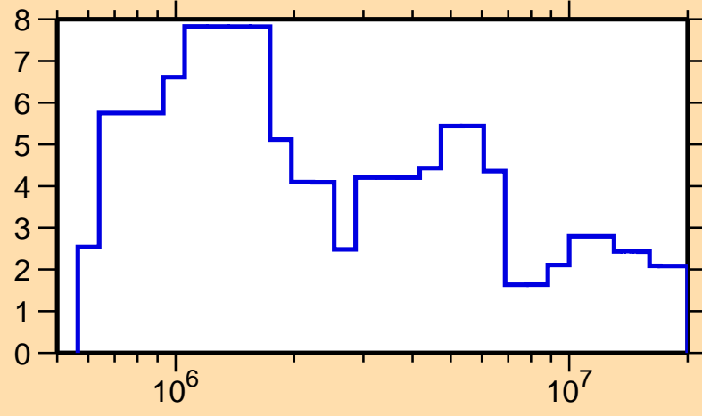
\Delta\sigma/\sigma vs. E for ^{179}\text{W}(n, el.)
