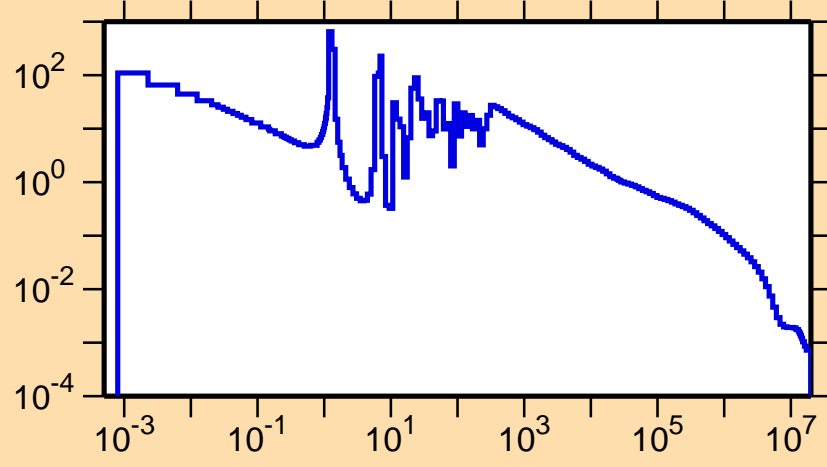
\sigma vs. E for ^{179}\text{W}(n,\gamma)
