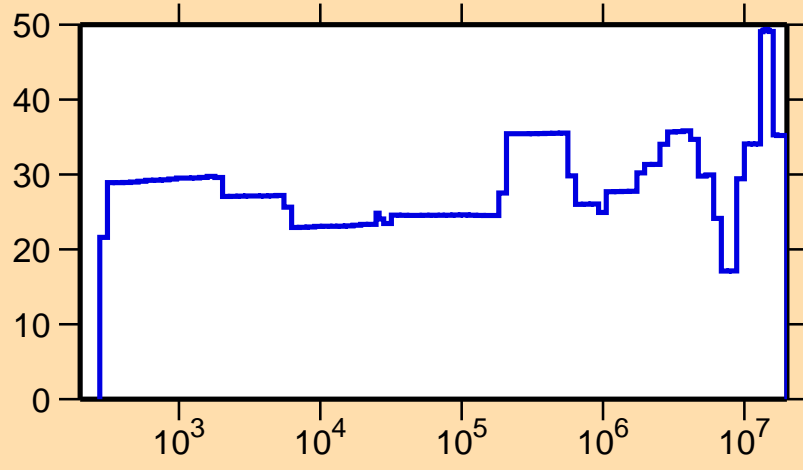
\Delta\sigma/\sigma vs. E for ^{179}\text{W}(n,\gamma)
