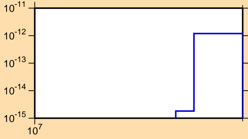
\sigma vs. E for ^{179}\text{W} (mt 34)
