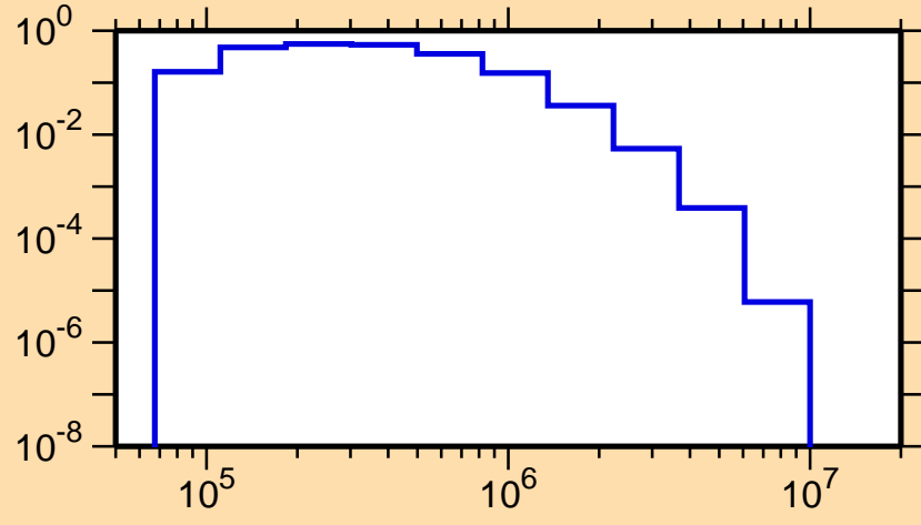
\sigma vs. E for ^{179}\text{W}(n,n_4)
