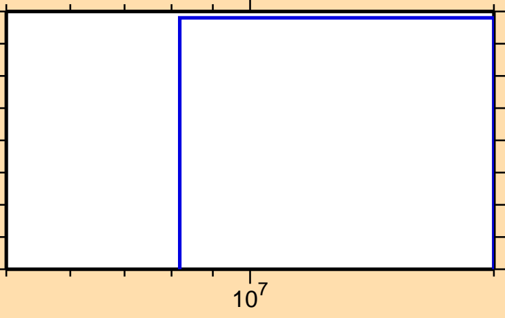
\sigma vs. E for ^{179}\text{W}(n,3n\alpha)
