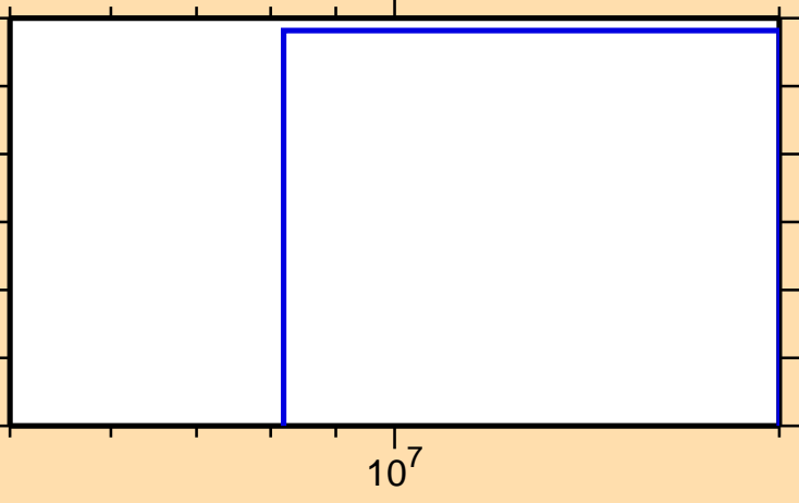
\sigma vs. E for ^{179}\text{W}(n,t)
