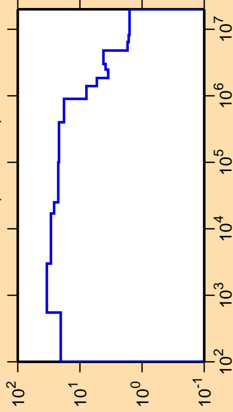
\Delta\sigma/\sigma vs. E for ^{179}\text{W}(n,\text{nonel.})
