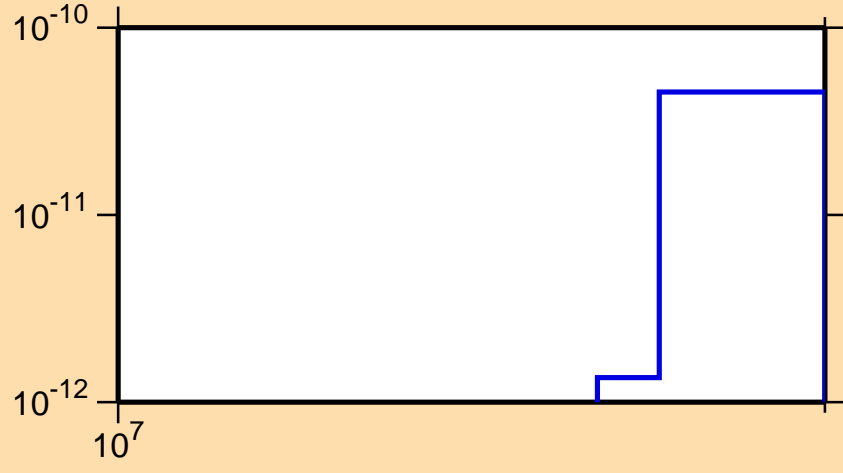
\sigma vs. E for ^{180}\text{W}(n,3n\alpha)
