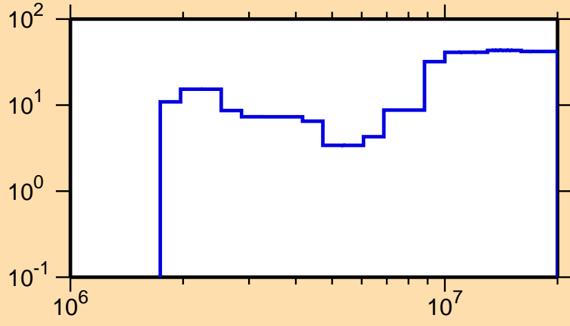
\Delta\sigma/\sigma vs. E for ^{180}\text{W}(n,n\text{cont.})
