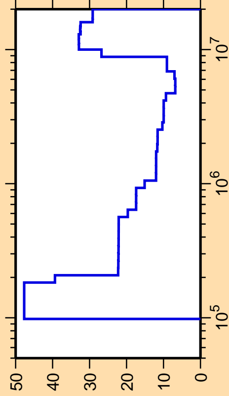
\Delta\sigma/\sigma vs. E for ^{180}\text{W}(n,\text{inel.})
