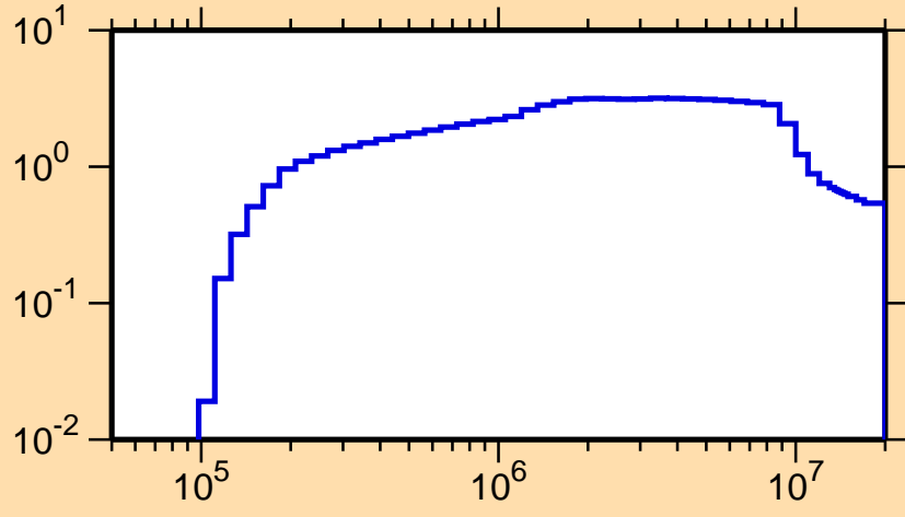
\sigma vs. E for ^{180}\text{W}(n,\text{inel.})
