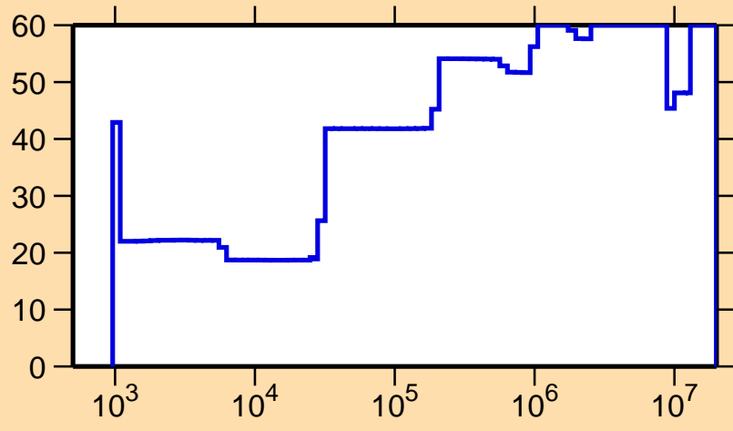
\Delta\sigma/\sigma vs. E for ^{180}\text{W}(n,\gamma)
