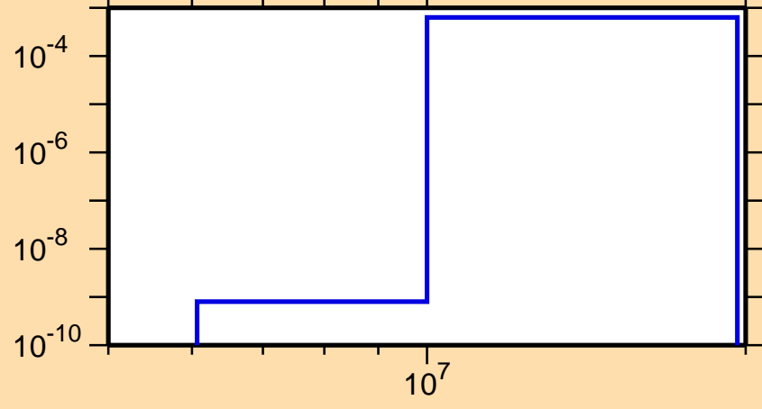
\sigma vs. E for ^{180}\text{W}(n,d)
