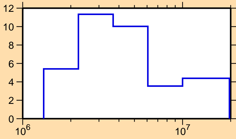
\Delta\sigma/\sigma vs. E for ^{180}\text{W}(n,el.)
