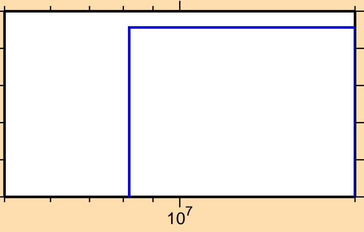
\sigma vs. E for ^{180}\text{W}(n,\text{nd})
