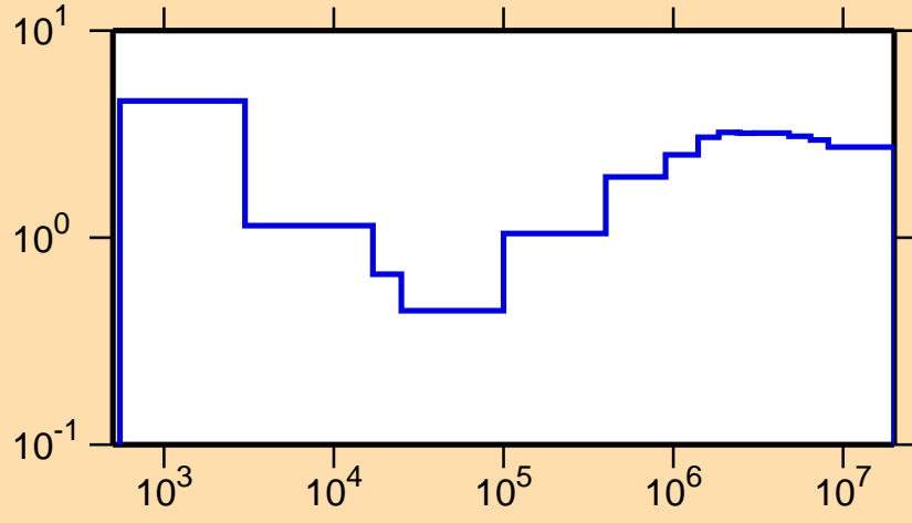
\sigma vs. E for ^{180}\text{W}(n,\text{nonel.})
