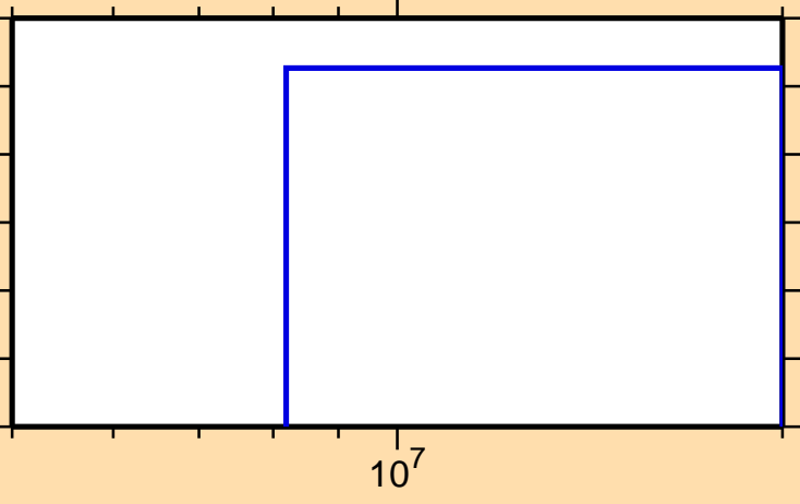
\sigma vs. E for ^{180}\text{W}(n,3n)
