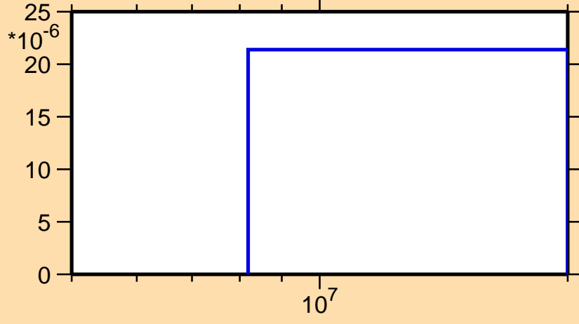
\sigma vs. E for ^{180}\text{W}(n,t)
