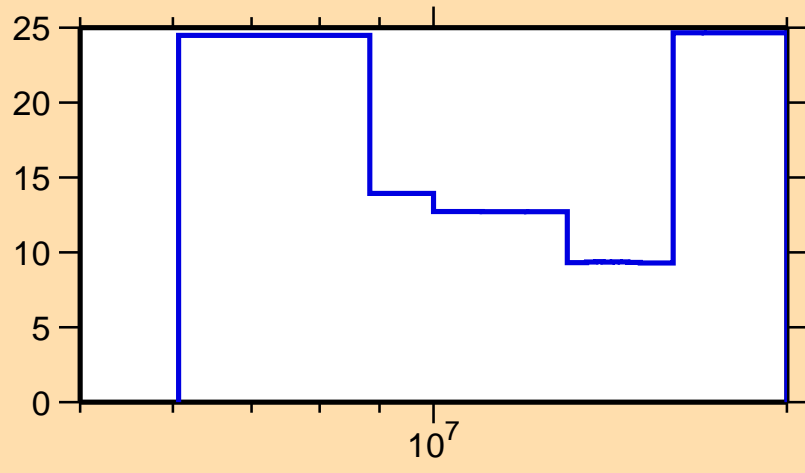
\Delta\sigma/\sigma vs. E for ^{181}\text{W}(n,2n)
