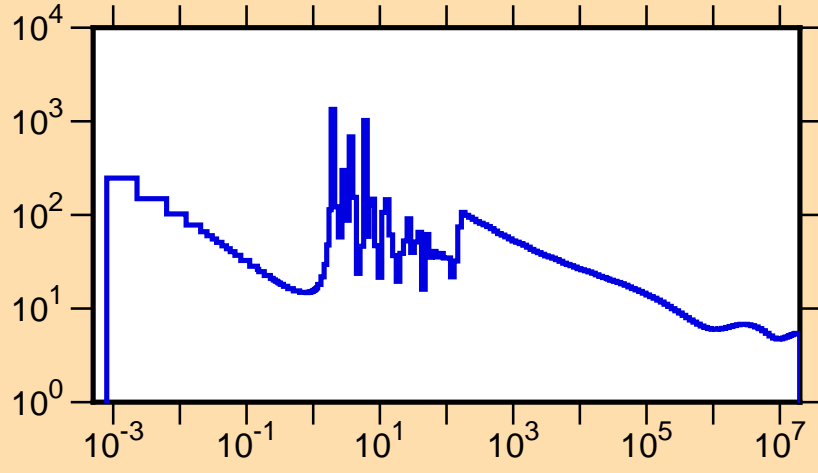
\sigma vs. E for ^{181}\text{W}(n,\text{tot.})
