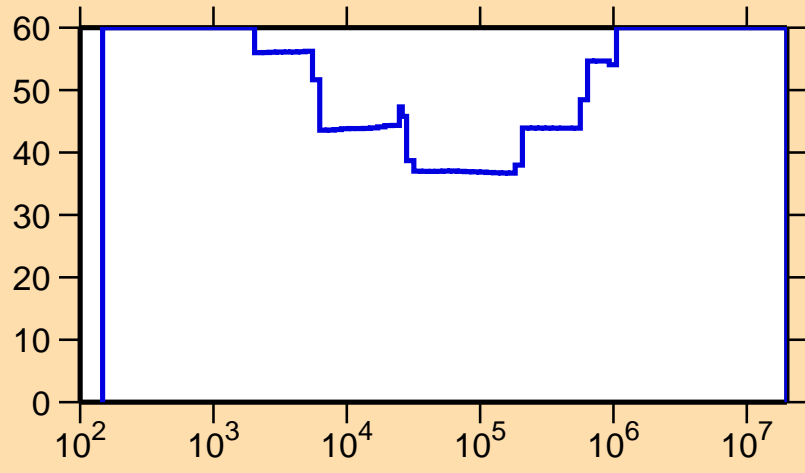
\Delta\sigma/\sigma vs. E for ^{181}\text{W}(n,\gamma)
