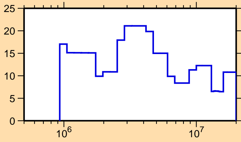
\Delta\sigma/\sigma vs. E for ^{181}\text{W}(n, el.)
