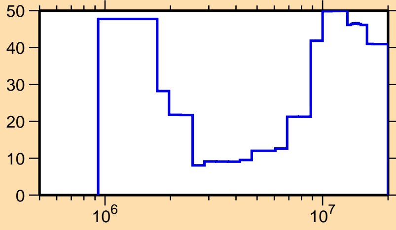
\Delta\sigma/\sigma vs. E for ^{181}\text{W}(n,ncont.)
