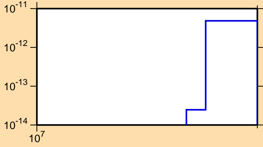
\sigma vs. E for ^{181}\text{W}(n,3n\alpha)
