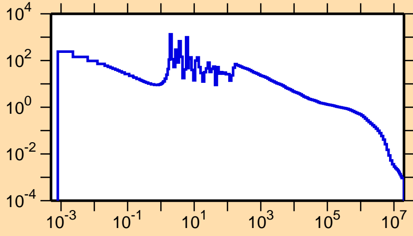
\sigma vs. E for ^{181}\text{W}(n,\gamma)
