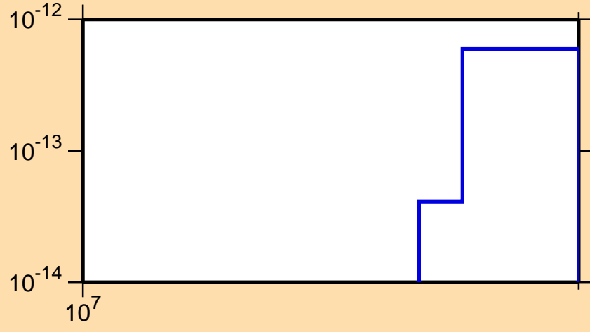
\sigma vs. E for ^{181}\text{W}(\text{mt117})
