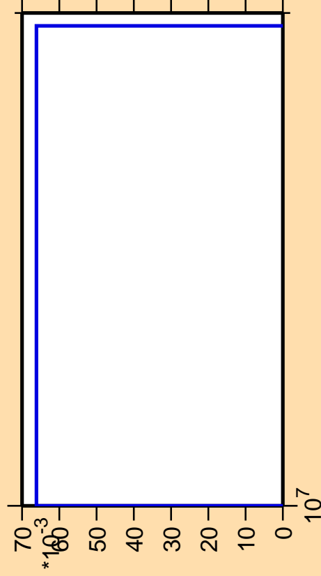
\Delta\sigma/\sigma vs. E for ^{181}\text{W}(\text{mt117})
