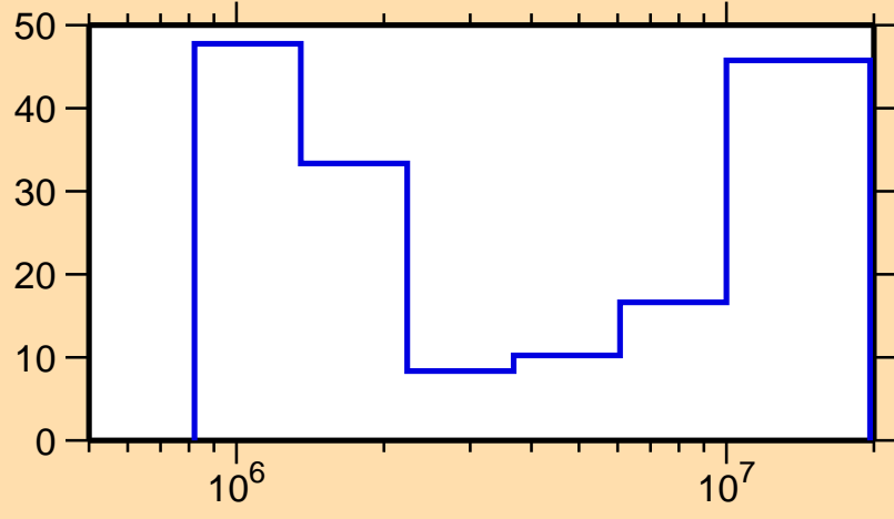
\Delta\sigma/\sigma vs. E for ^{181}\text{W}(n,n\text{cont.})
