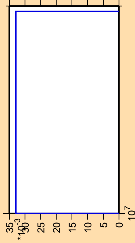
\Delta\sigma/\sigma vs. E for ^{181}\text{W} (mt 45)
