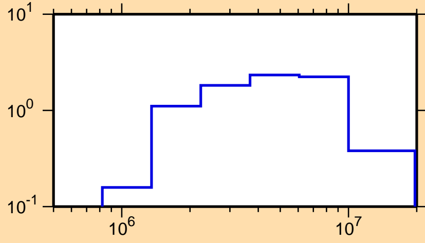
\sigma vs. E for ^{181}\text{W}(n,n\text{cont.})
