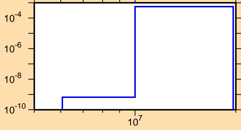
\sigma vs. E for ^{181}\text{W}(n,d)
