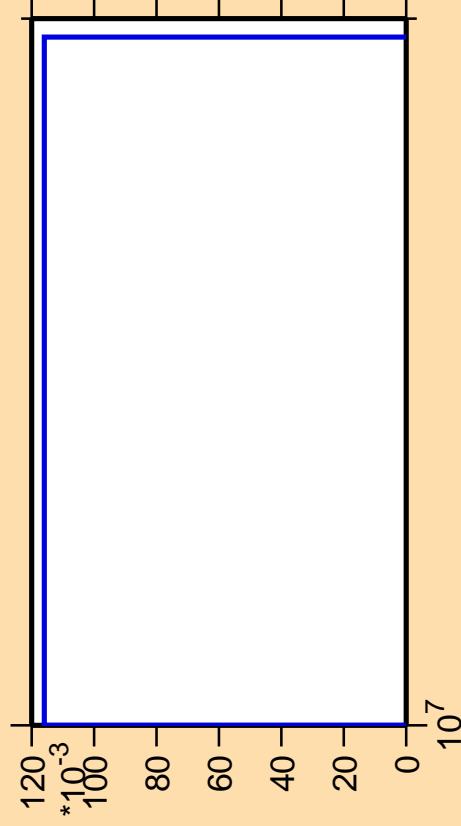
\Delta\sigma/\sigma vs. E for ^{181}\text{W}(n,3n\alpha)
