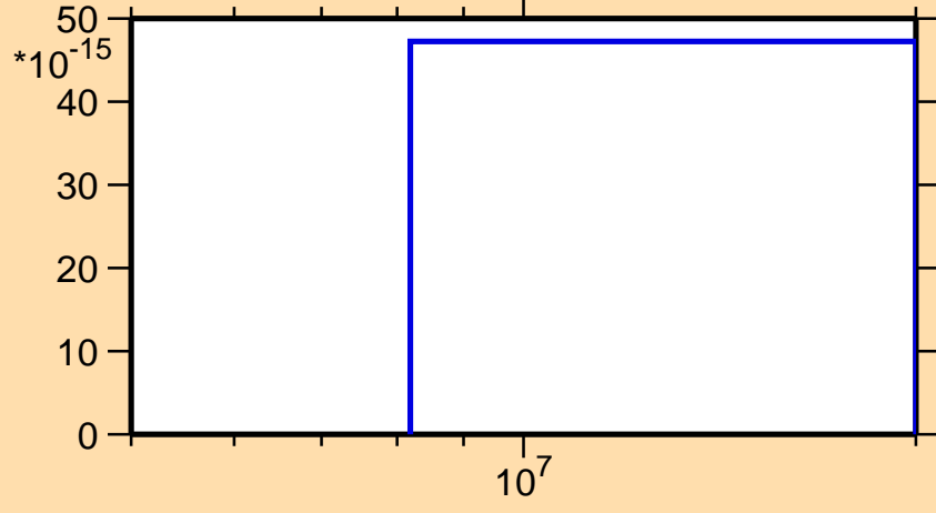
\sigma vs. E for ^{181}\text{W}(n,3n\alpha)
