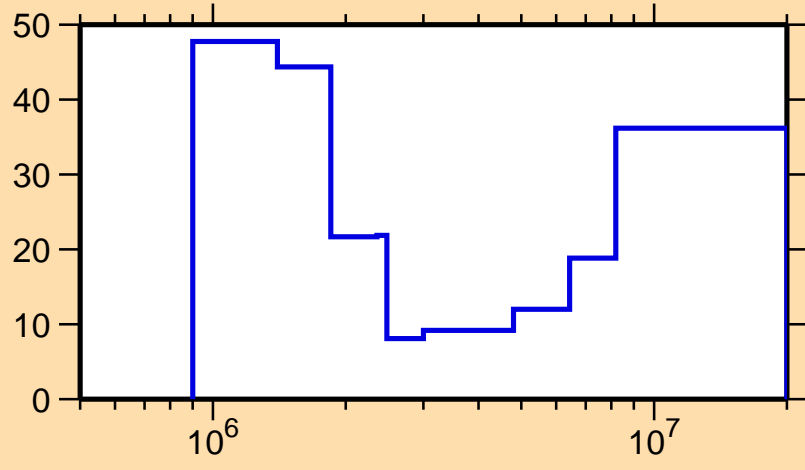
\Delta\sigma/\sigma vs. E for ^{181}\text{W}(n,n\text{cont.})
