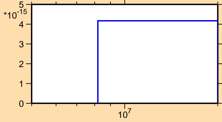
\sigma vs. E for ^{181}\text{W} (mt 45)
