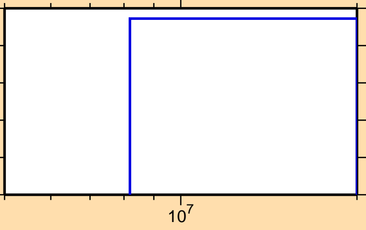
\sigma vs. E for ^{181}\text{W}(n,3n\alpha)
