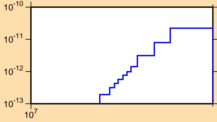
\sigma vs. E for ^{182}\text{W}(n,p\alpha)
