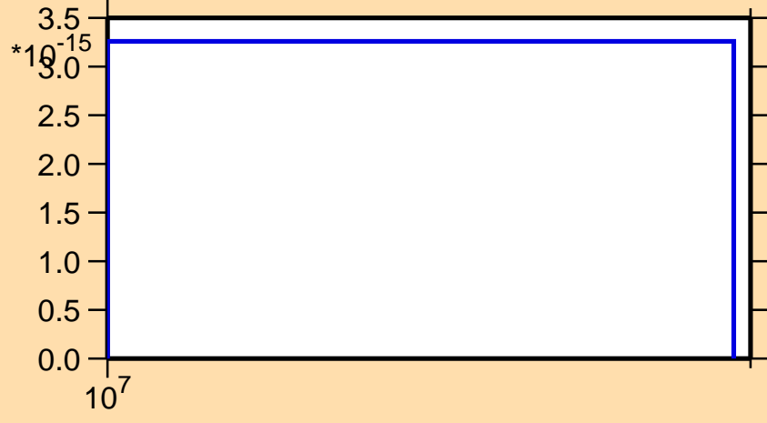
\sigma vs. E for ^{182}\text{W}(\text{mt117})
