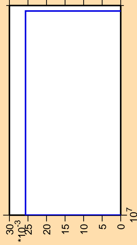
\Delta\sigma/\sigma vs. E for ^{182}\text{W}(\text{mt117})
