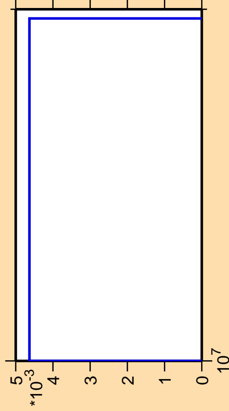
\Delta\sigma/\sigma vs. E for ^{182}\text{W} (mt 45)
