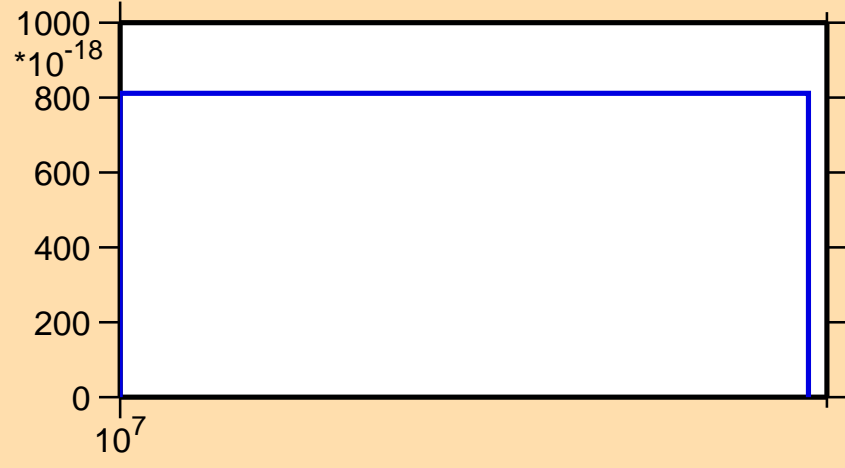
\sigma vs. E for ^{182}\text{W} (mt 45)
