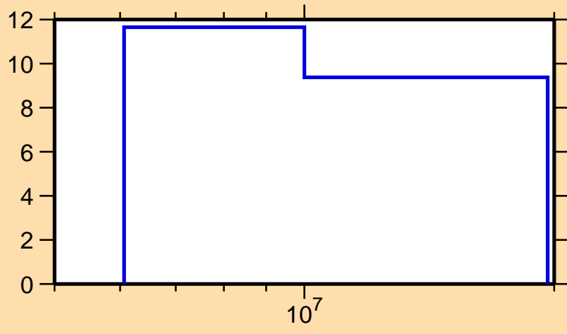
\Delta\sigma/\sigma vs. E for ^{182}\text{W}(n,2n)
