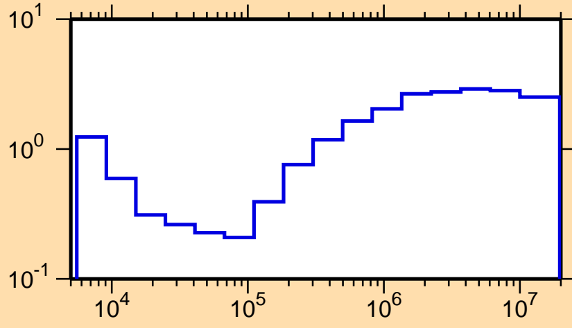
\sigma vs. E for ^{182}\text{W}(n,\text{nonel.})
