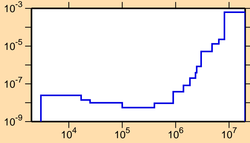
\sigma vs. E for ^{182}\text{W}(n,\alpha)
