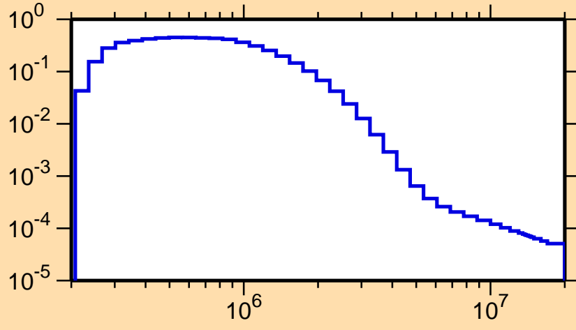
\sigma vs. E for ^{183}\text{W}(n,n_4)
