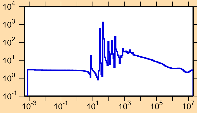
\sigma vs. E for ^{183}\text{W}(n,\text{el.})
