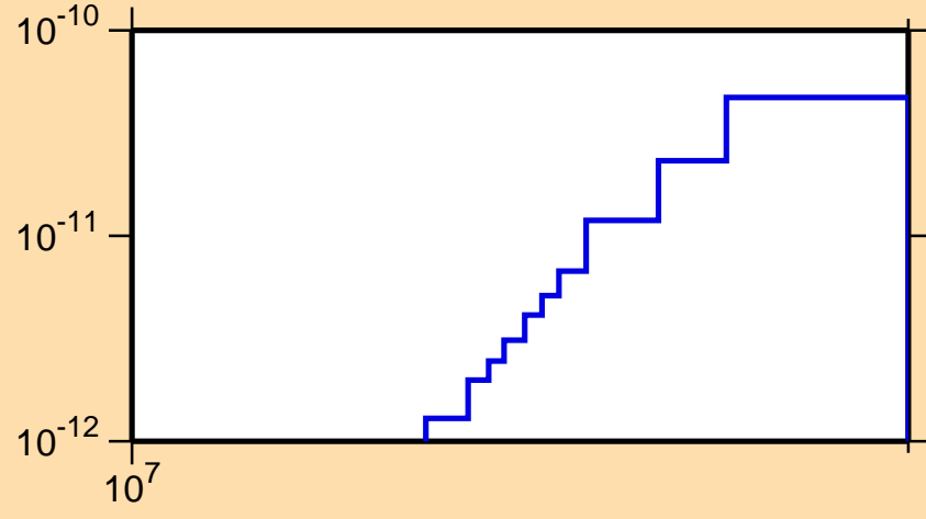
\sigma vs. E for ^{183}\text{W}(n,p\alpha)
