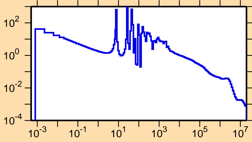
\sigma vs. E for ^{183}\text{W}(n,\gamma)
