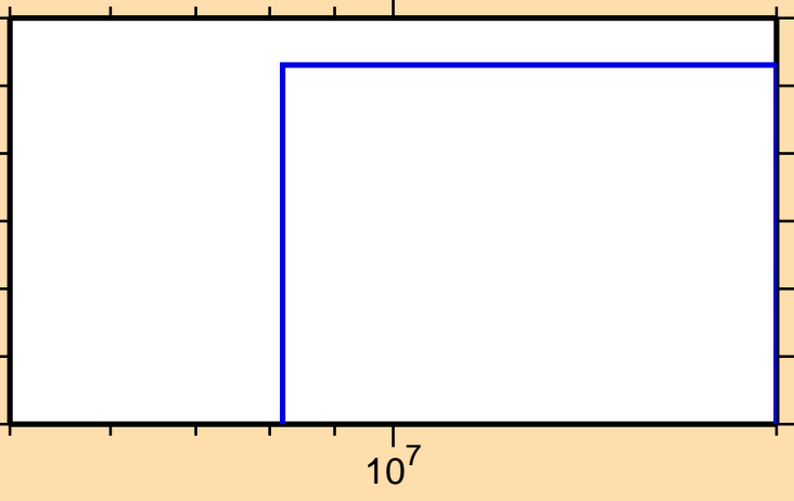
\sigma vs. E for ^{183}\text{W}(n,2n\alpha)
