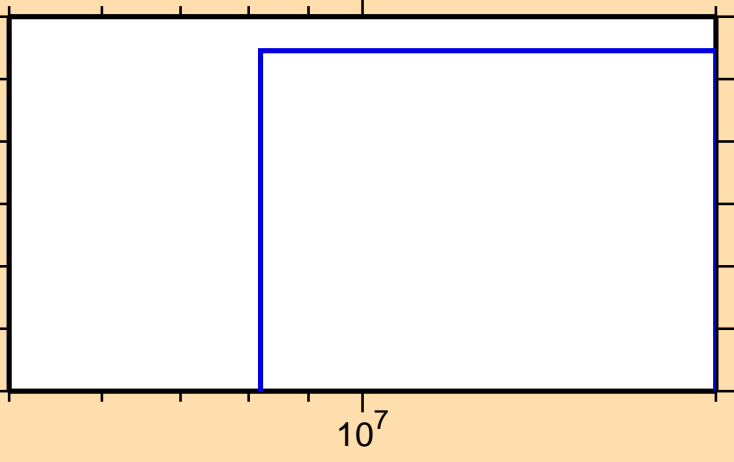
\sigma vs. E for ^{183}\text{W}(n,3n)
