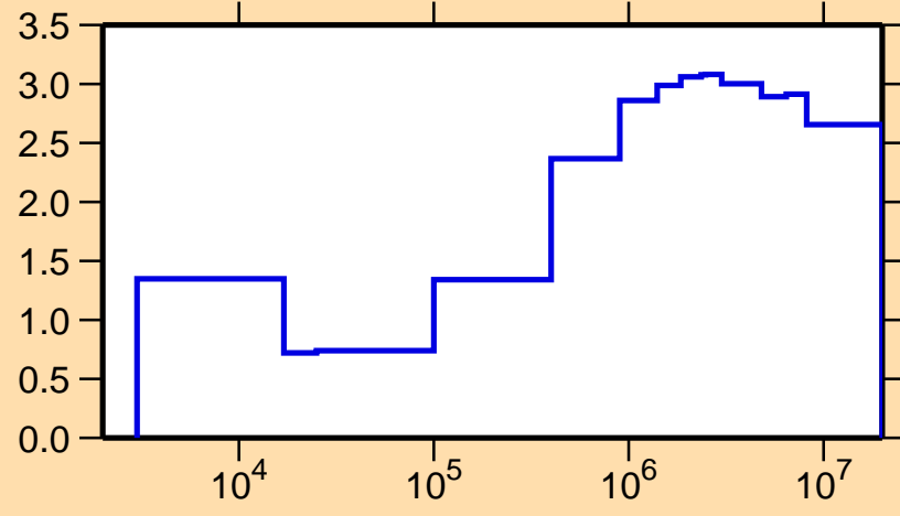
\sigma vs. E for ^{183}\text{W}(n,\text{nonel.})
