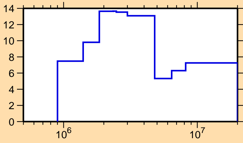
\Delta\sigma/\sigma vs. E for ^{183}\text{W}(n, el.)
