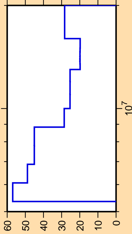
\Delta\sigma/\sigma vs. E for ^{183}\text{W}(n,2n)
