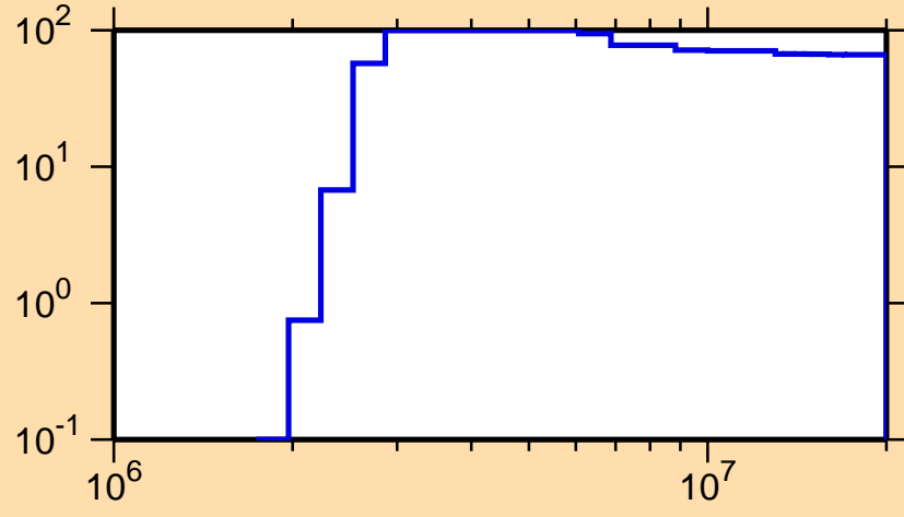
\Delta\sigma/\sigma vs. E for ^{183}\text{W}(n,p)
