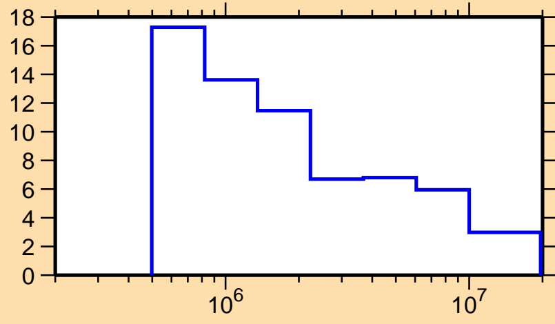
\Delta\sigma/\sigma vs. E for ^{183}\text{W}(n, tot.)
