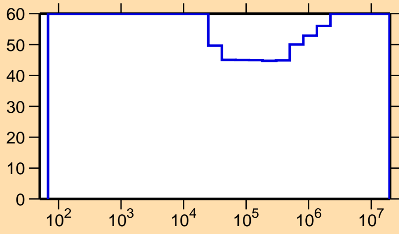
\Delta\sigma/\sigma vs. E for ^{183}\text{W}(n,\gamma)
