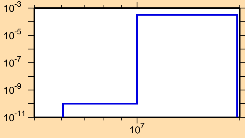
\sigma vs. E for ^{183}\text{W}(n,d)
