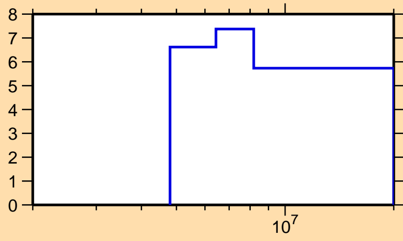
\Delta\sigma/\sigma vs. E for ^{183}\text{W}(n,\text{nonel.})
