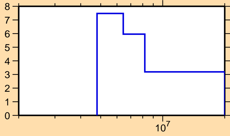
\Delta\sigma/\sigma vs. E for ^{183}\text{W}(n,\text{tot.})
