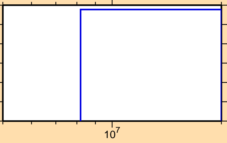
\sigma vs. E for ^{183}\text{W}(n,\text{nd})
