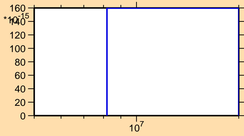
\sigma vs. E for ^{184}\text{W}(n,p\alpha)
