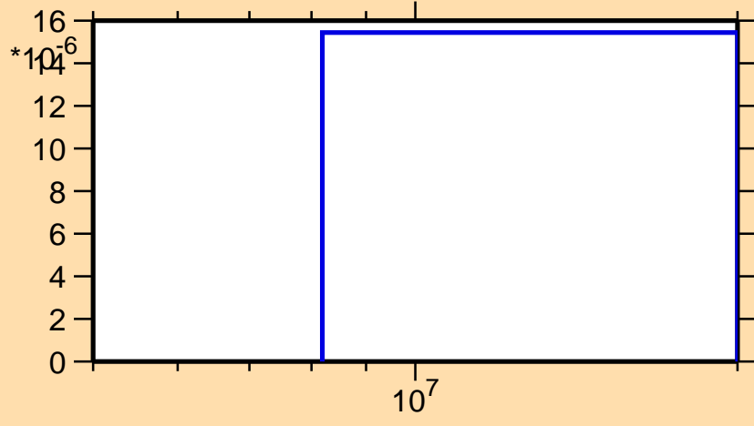
\sigma vs. E for ^{184}\text{W}(n,t)
