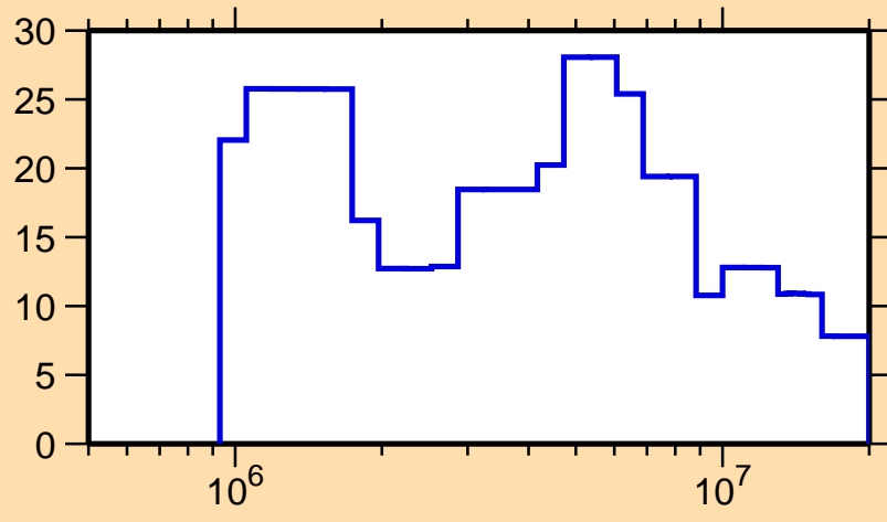
\Delta\sigma/\sigma vs. E for ^{185}\text{W}(n, el.)
