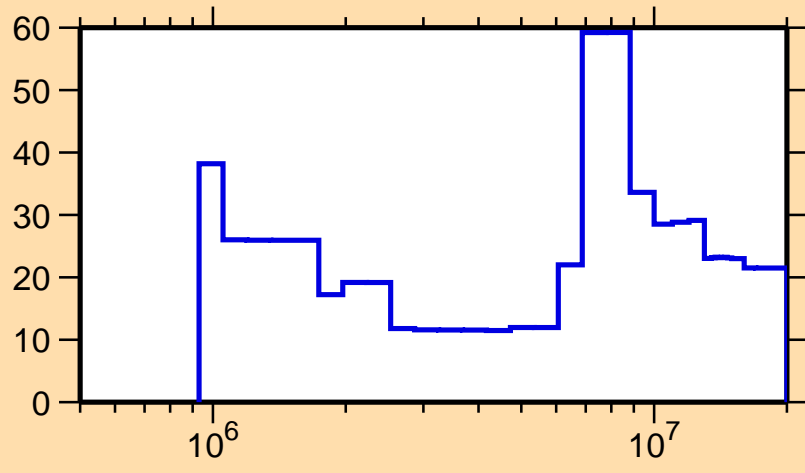
\Delta\sigma/\sigma vs. E for ^{185}\text{W}(n,n\text{cont.})
