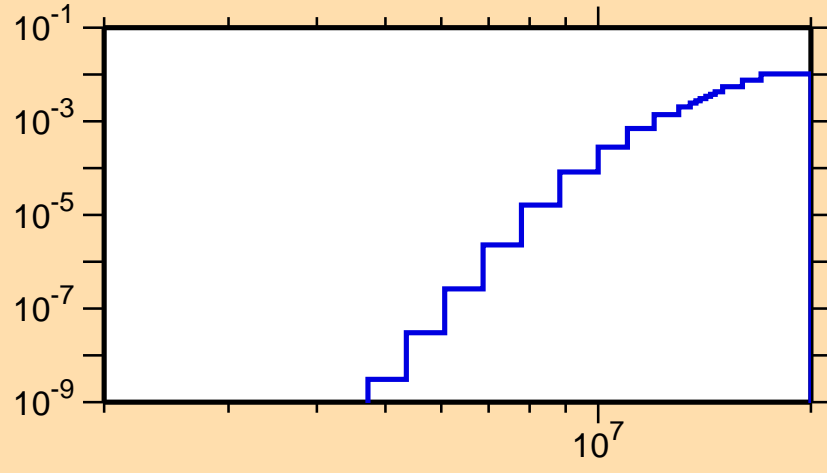
\sigma vs. E for ^{185}\text{W}(n,p)
