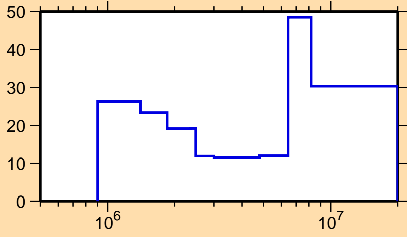
\Delta\sigma/\sigma vs. E for ^{185}\text{W}(n,n\text{cont.})
