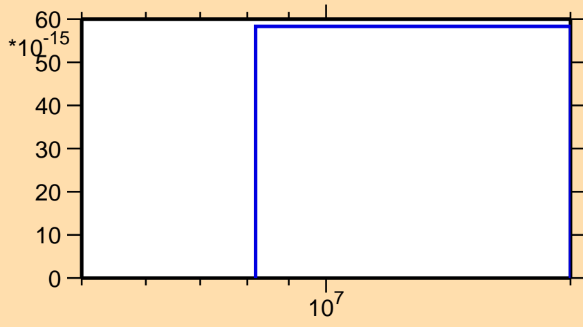
\sigma vs. E for ^{185}\text{W}(n,3n\alpha)
