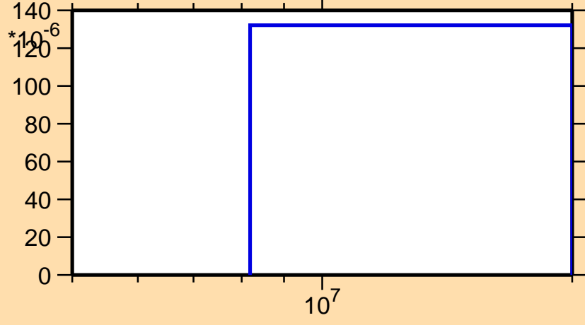
\sigma vs. E for ^{185}\text{W}(n,d)
