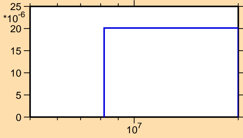
\sigma vs. E for ^{185}\text{W}(n,t)
