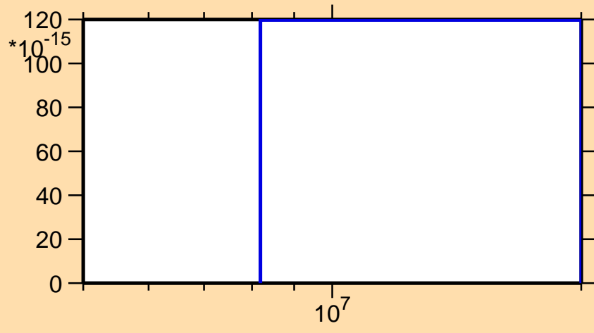
\sigma vs. E for ^{185}\text{W}(n,p\alpha)
