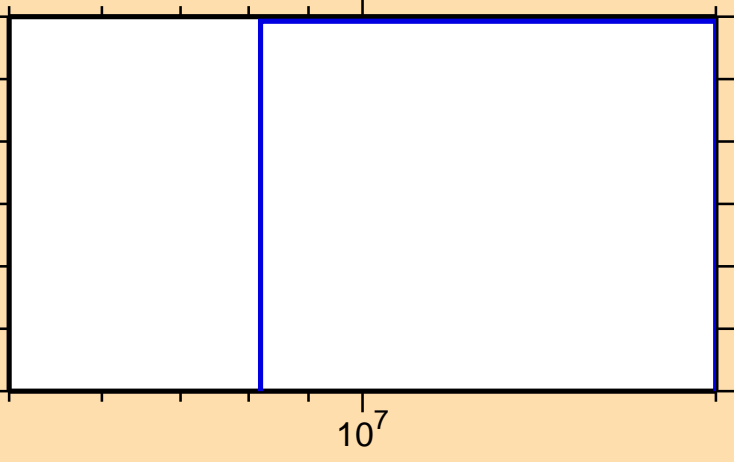
\sigma vs. E for ^{185}\text{W}(n,2n\alpha)
