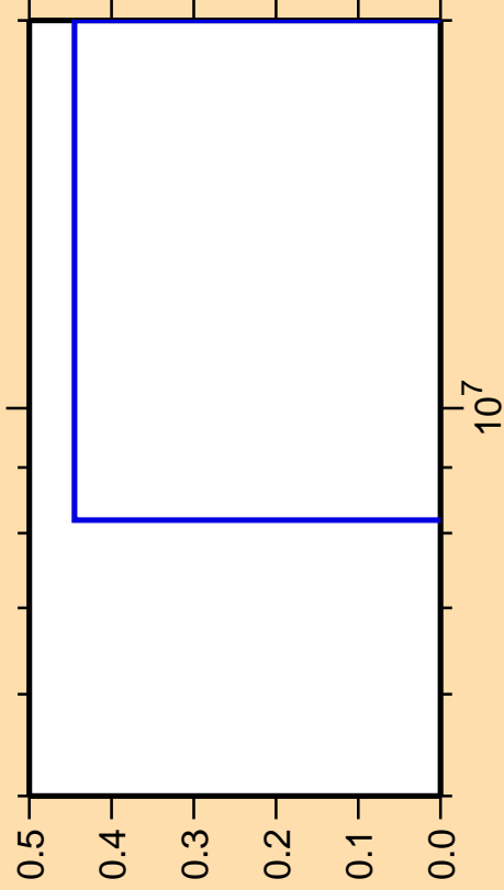
\Delta\sigma/\sigma vs. E for ^{185}\text{W}(n,p\alpha)
