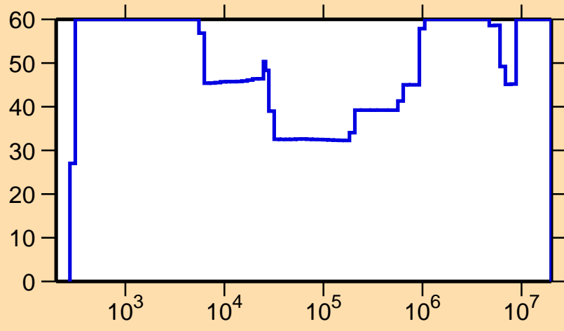
\Delta\sigma/\sigma vs. E for ^{185}\text{W}(n,\gamma)
