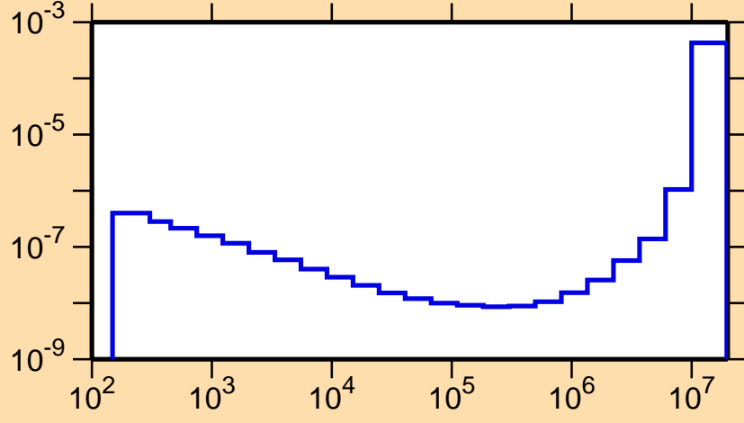
\sigma vs. E for ^{185}\text{W}(n,\alpha)
