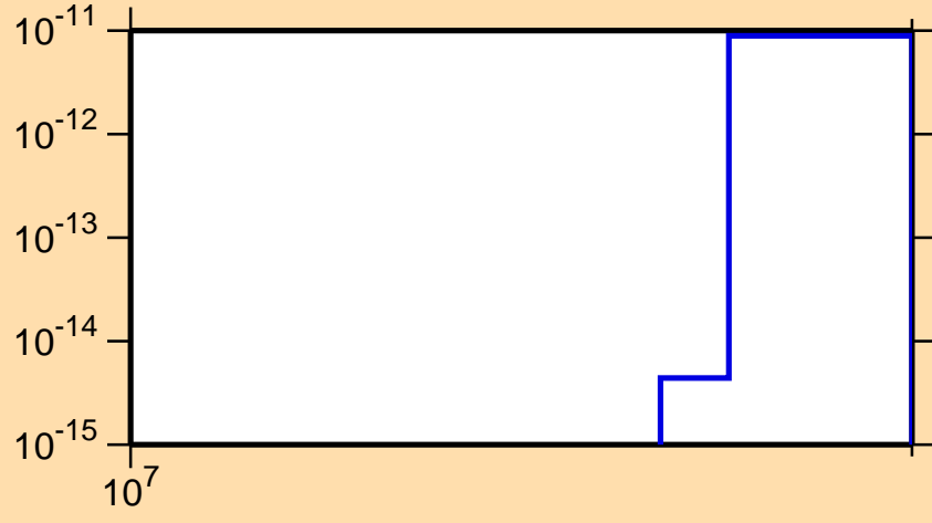
\sigma vs. E for ^{186}\text{W}(n,3n\alpha)
