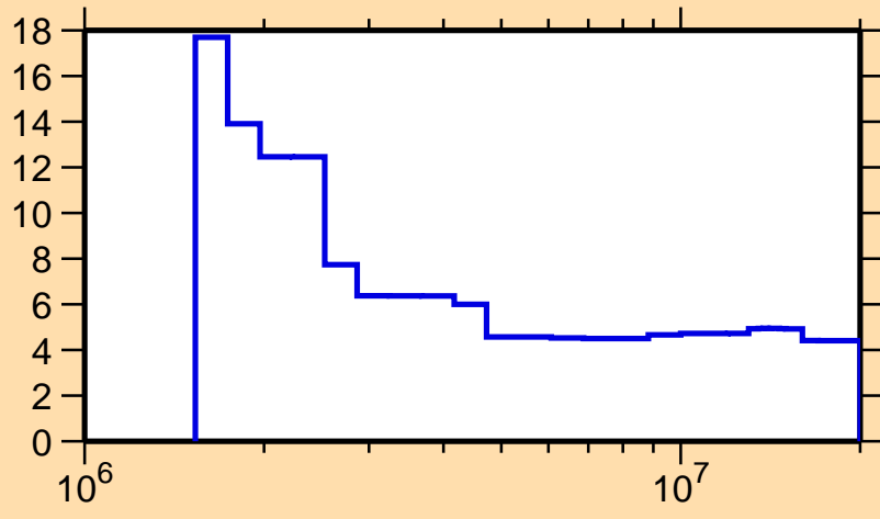
\Delta\sigma/\sigma vs. E for ^{186}\text{W}(n,n\text{onel.})
