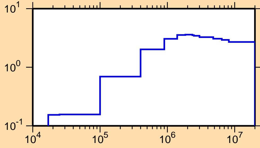
\sigma vs. E for ^{186}\text{W}(n,\text{nonel.})
