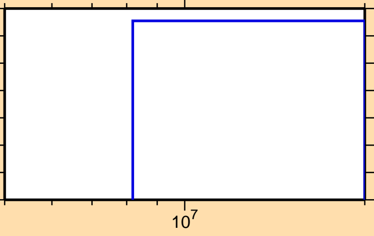
\sigma vs. E for ^{186}\text{W}(n,2n\alpha)
