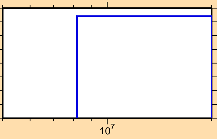
\sigma vs. E for ^{186}\text{W}(n,3n\alpha)
