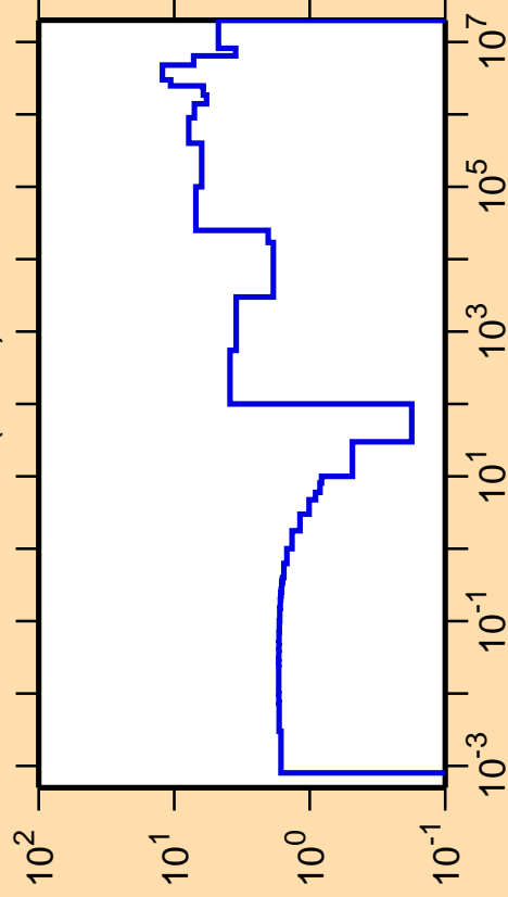
\Delta\sigma/\sigma vs. E for ^{186}\text{W}(n,\text{el.})
