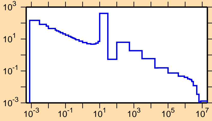
\sigma vs. E for ^{186}\text{W}(n,\gamma)
