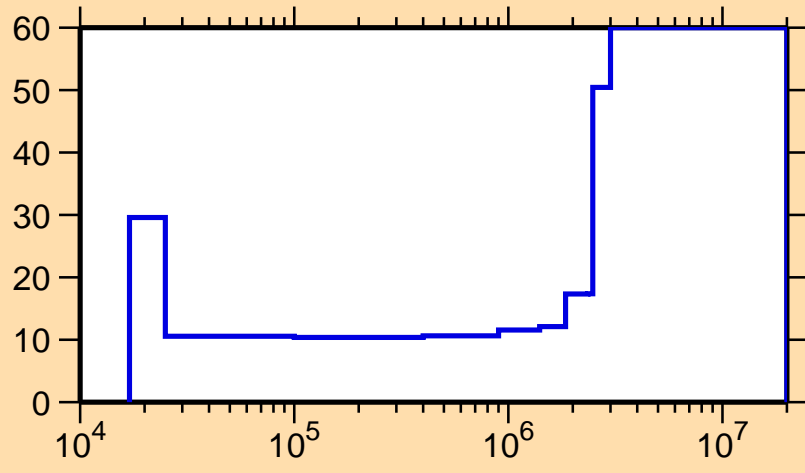
\Delta\sigma/\sigma vs. E for ^{186}\text{W}(n,\gamma)
