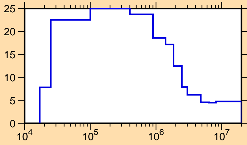
\Delta\sigma/\sigma vs. E for ^{186}\text{W}(n,\text{nonel.})
