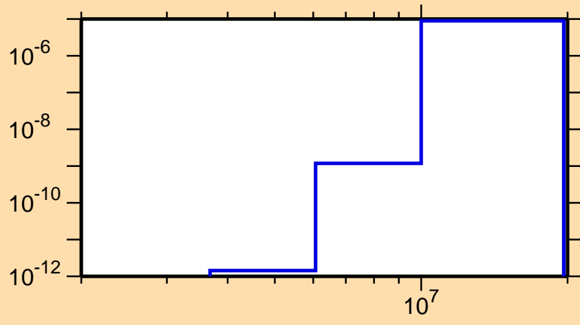
\sigma vs. E for ^{187}\text{W}(n,n\alpha)
