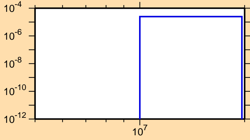
\sigma vs. E for ^{187}\text{W}(n,np)
