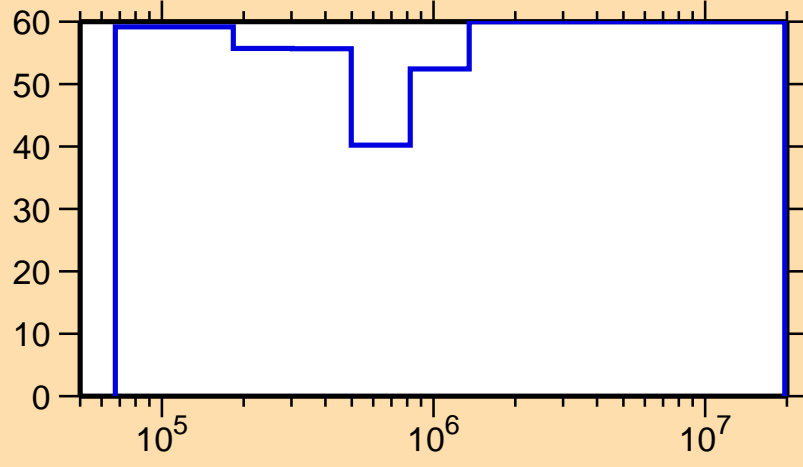
\Delta\sigma/\sigma vs. E for ^{187}\text{W}(n,n_1)
