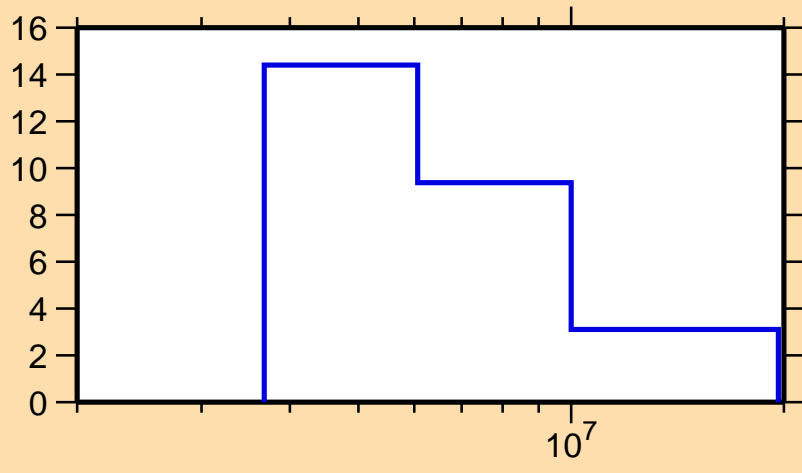
\Delta\sigma/\sigma vs. E for ^{187}\text{W}(n,\text{tot.})
