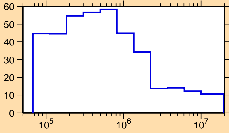
\Delta\sigma/\sigma vs. E for ^{187}\text{W}(n,\text{nonel.})
