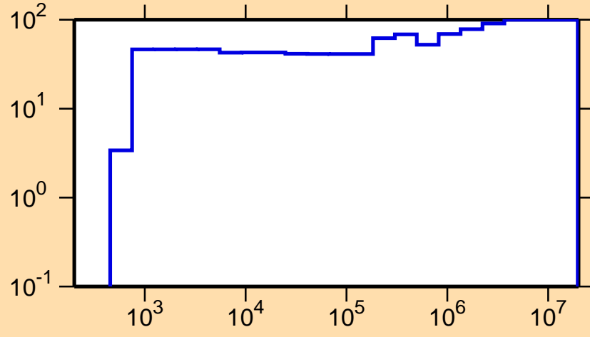
\Delta\sigma/\sigma vs. E for ^{187}\text{W}(n,\gamma)
