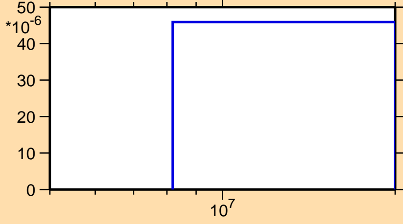
\sigma vs. E for ^{187}\text{W}(n,d)
