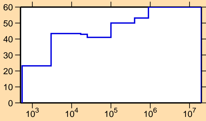
\Delta\sigma/\sigma vs. E for ^{187}\text{W}(n,\gamma)
