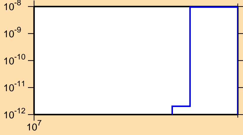
\sigma vs. E for ^{188}\text{W}(n,\text{nd})
