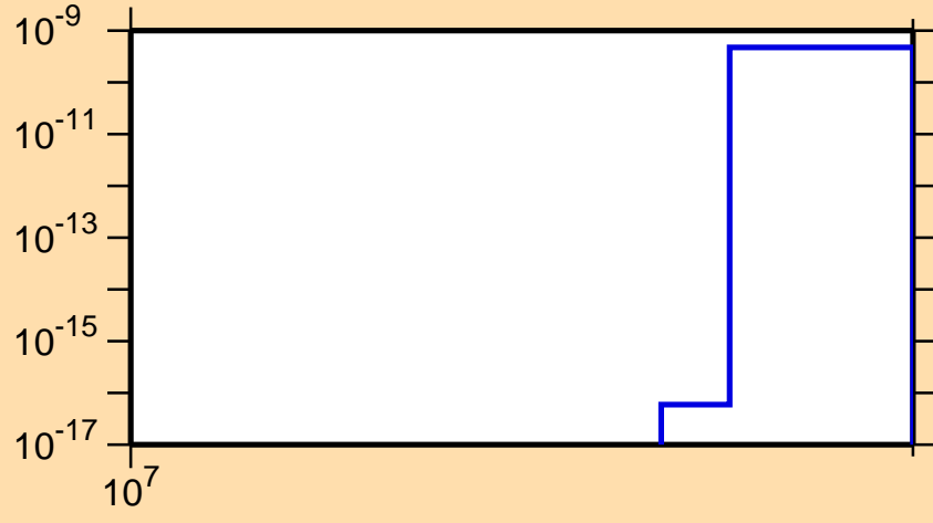
\sigma vs. E for ^{188}\text{W}(n,2np)
