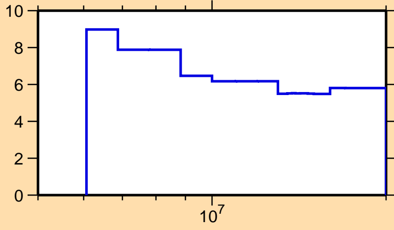
\Delta\sigma/\sigma vs. E for ^{188}\text{W}(n,\text{nonel.})
