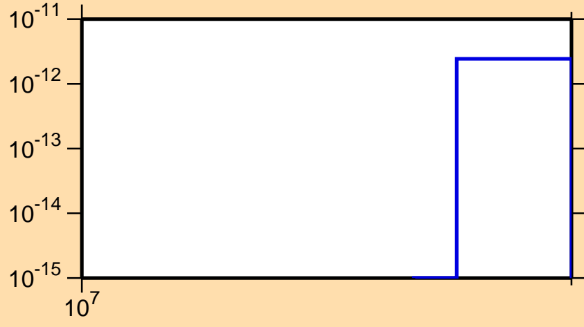
\sigma vs. E for ^{188}\text{W}(n,3n\alpha)
