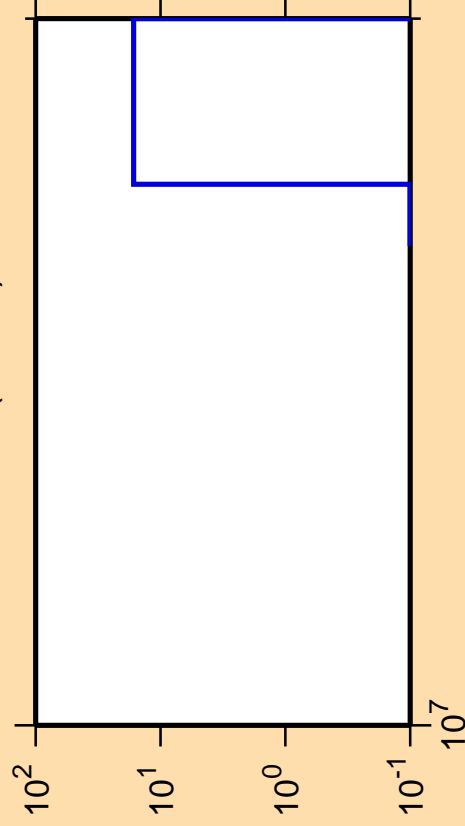
\Delta\sigma/\sigma vs. E for ^{188}\text{W}(n,3n\alpha)
