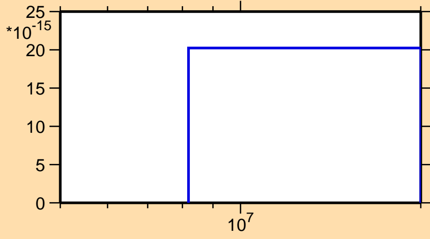
\sigma vs. E for ^{188}\text{W}(n,3n\alpha)
