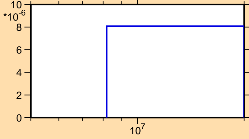
\sigma vs. E for ^{188}\text{W}(n,np)
