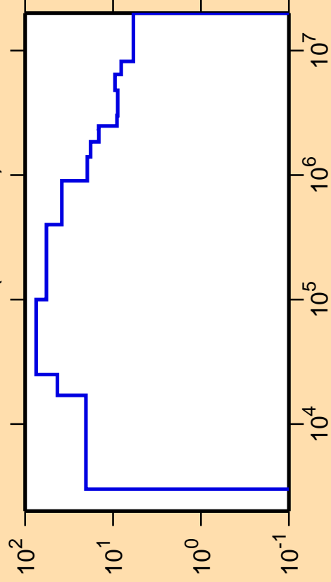
\Delta\sigma/\sigma vs. E for ^{188}\text{W}(n,\text{nonel.})
