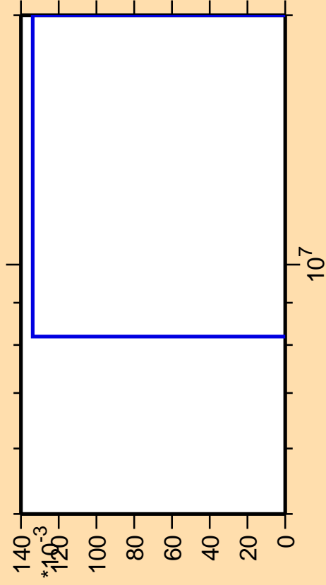
\Delta\sigma/\sigma vs. E for ^{188}\text{W}(n,3n\alpha)
