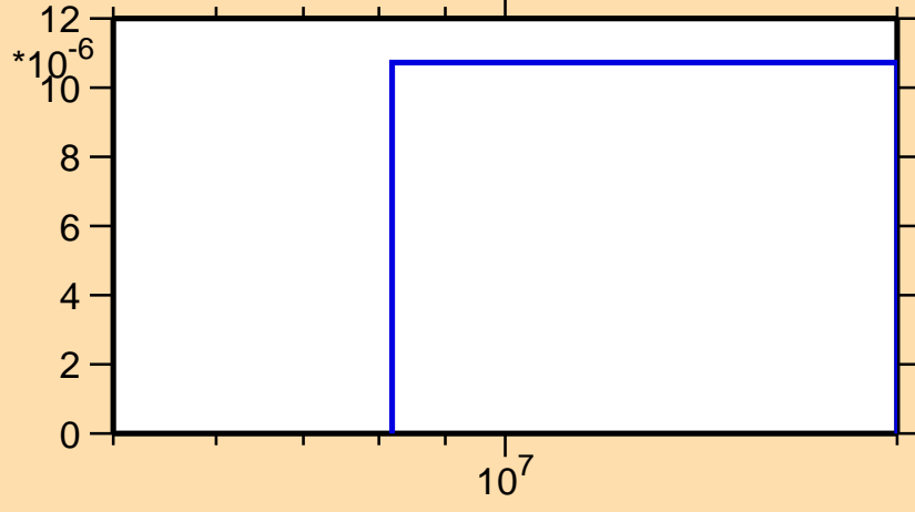
\sigma vs. E for ^{188}\text{W}(n,d)
