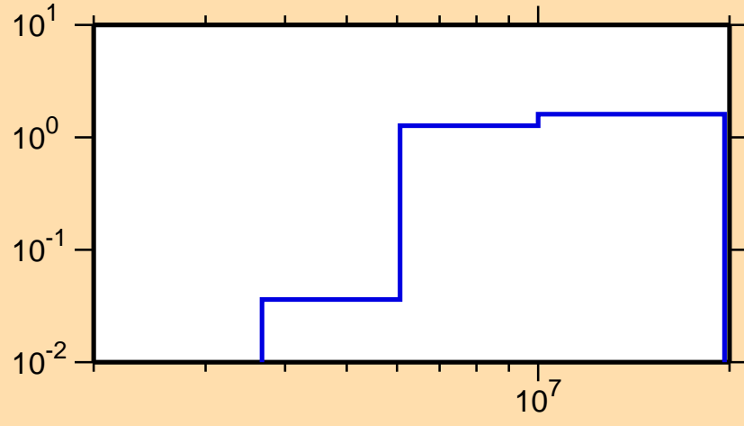
\sigma vs. E for ^{189}\text{W}(n,2n)
