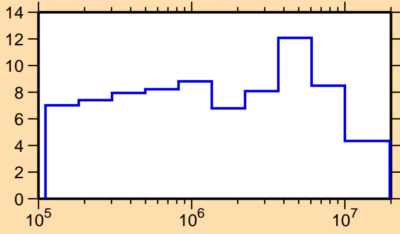
\Delta\sigma/\sigma vs. E for ^{189}\text{W}(n, el.)
