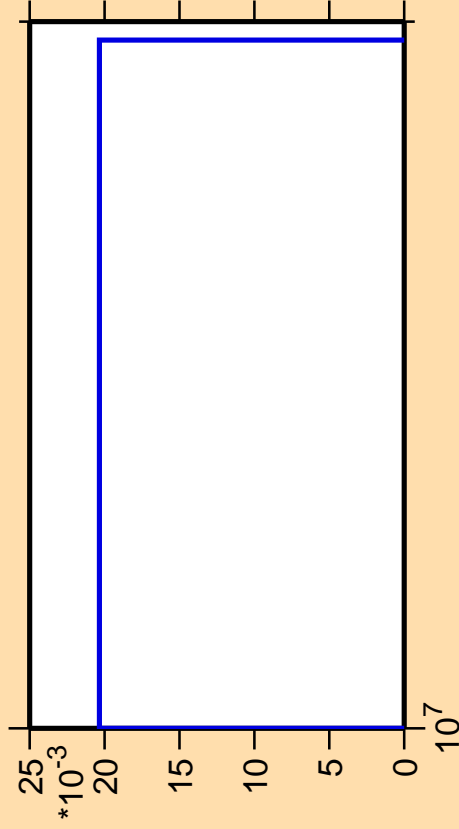
\Delta\sigma/\sigma vs. E for ^{189}\text{W}(n,3n\alpha)
