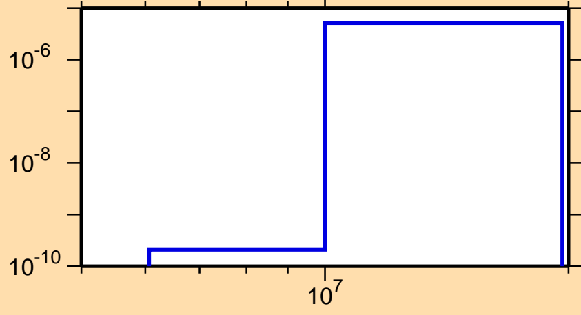
\sigma vs. E for ^{189}\text{W}(n,n\alpha)
