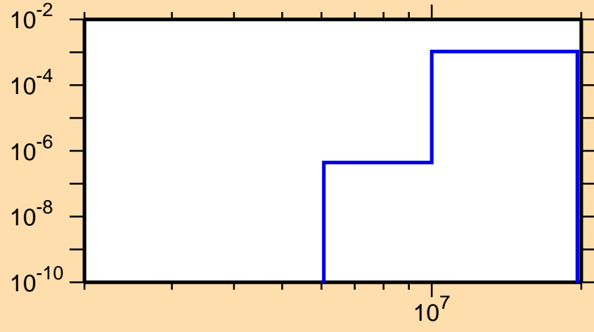
\sigma vs. E for ^{189}\text{W}(n,p)
