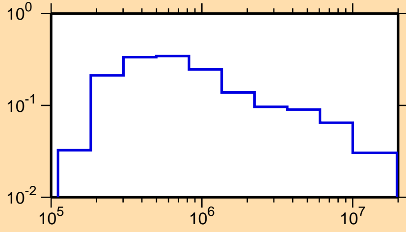
\sigma vs. E for ^{189}\text{W}(n,n_1)
