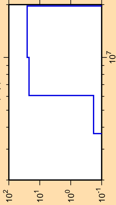
\Delta\sigma/\sigma vs. E for ^{189}\text{W}(n,p)
