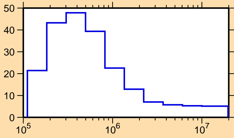
\Delta\sigma/\sigma vs. E for ^{189}\text{W}(n,\text{nonel.})
