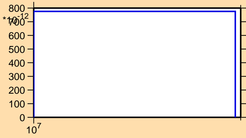
\sigma vs. E for ^{189}\text{W}(n,nt)
