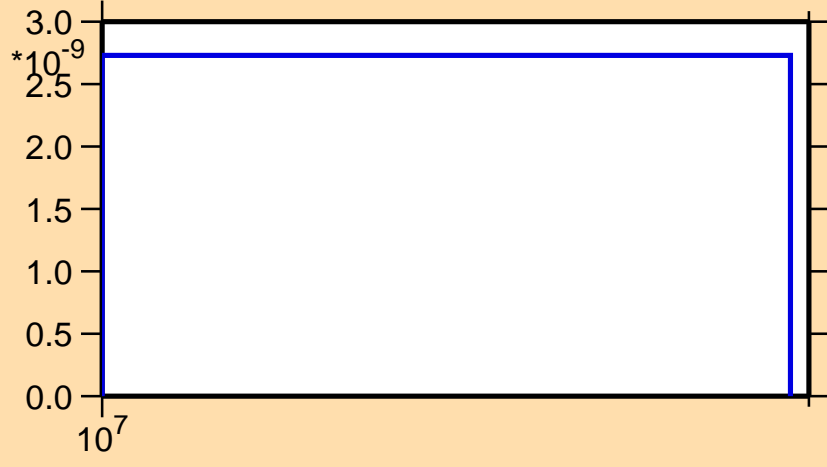
\sigma vs. E for ^{189}\text{W}(n,\text{nd})
