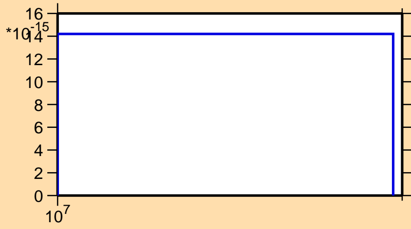
\sigma vs. E for ^{189}\text{W}(n,3n\alpha)
