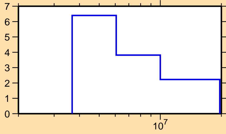
\Delta\sigma/\sigma vs. E for ^{189}\text{W}(n,\text{tot.})
