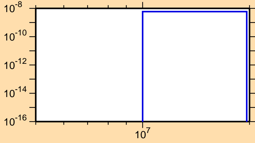
\sigma vs. E for ^{189}\text{W}(n,2n\alpha)
