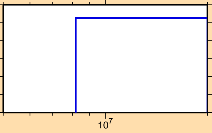
\sigma vs. E for ^{189}\text{W}(n,\text{nd})
