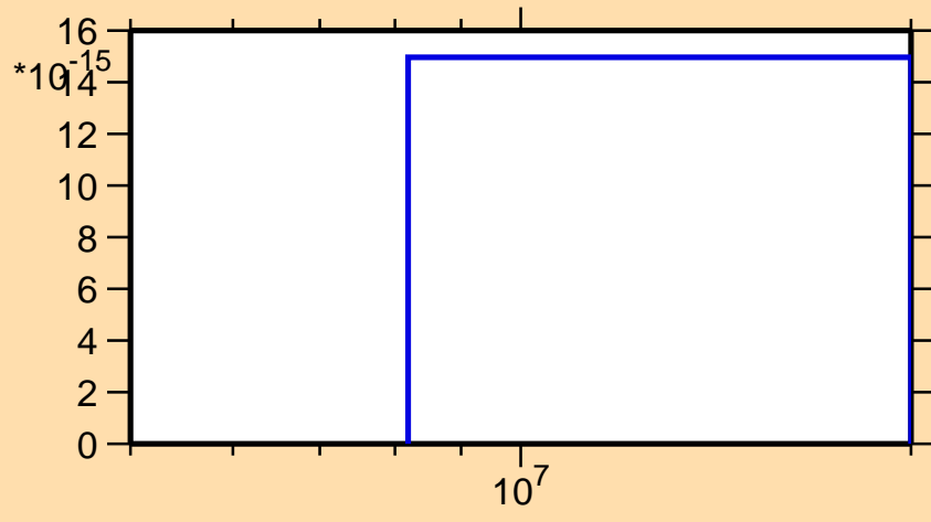
\sigma vs. E for ^{189}\text{W}(n,3n\alpha)
