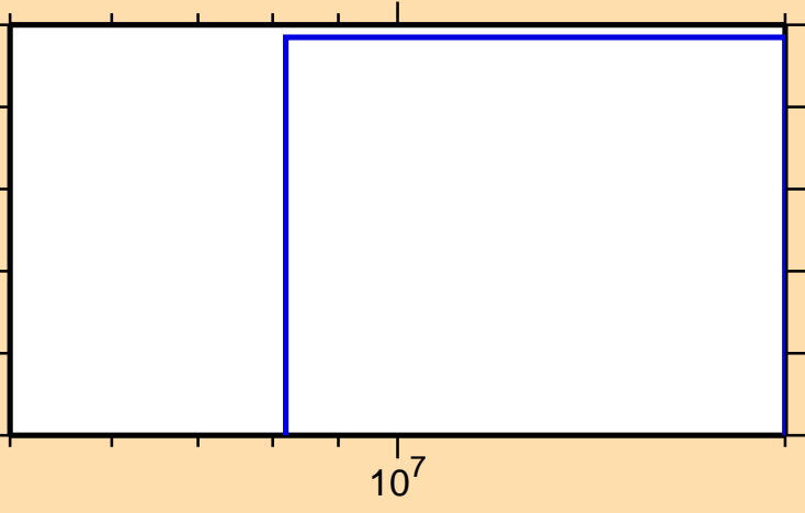
\sigma vs. E for ^{189}\text{W}(n,2n\alpha)
