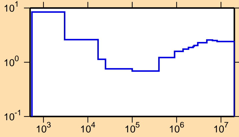
\sigma vs. E for ^{189}\text{W}(n,\text{nonel.})
