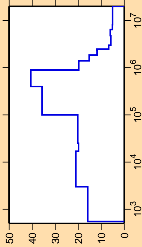
\Delta\sigma/\sigma vs. E for ^{189}\text{W}(n,\text{nonel.})
