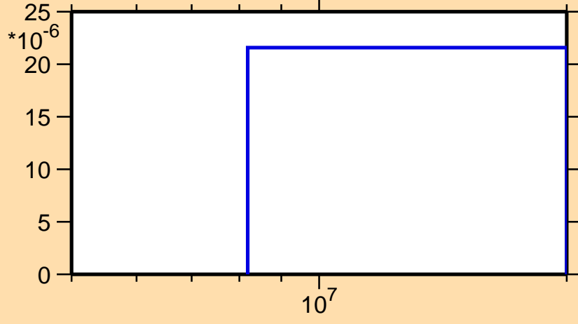
\sigma vs. E for ^{189}\text{W}(n,d)
