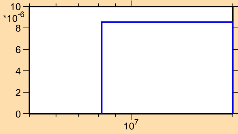
\sigma vs. E for ^{189}\text{W}(n,t)
