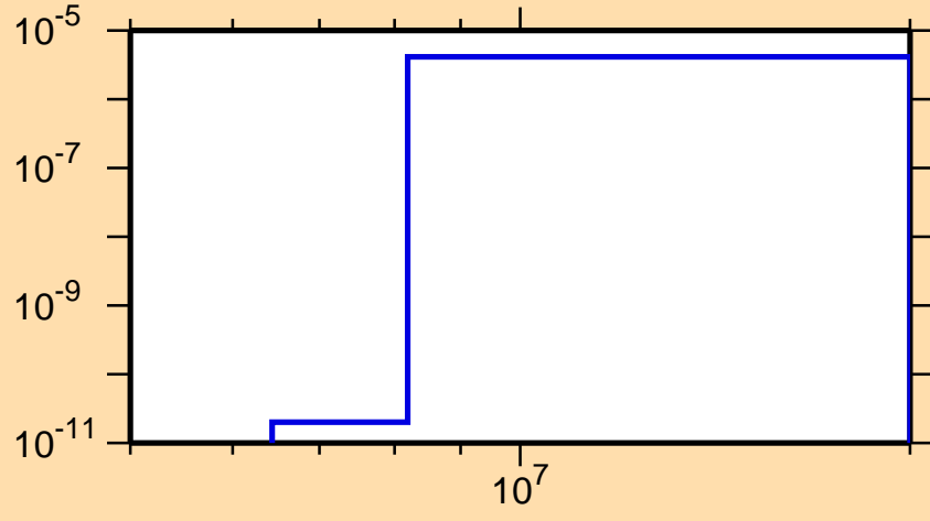
\sigma vs. E for ^{189}\text{W}(n,n\alpha)
