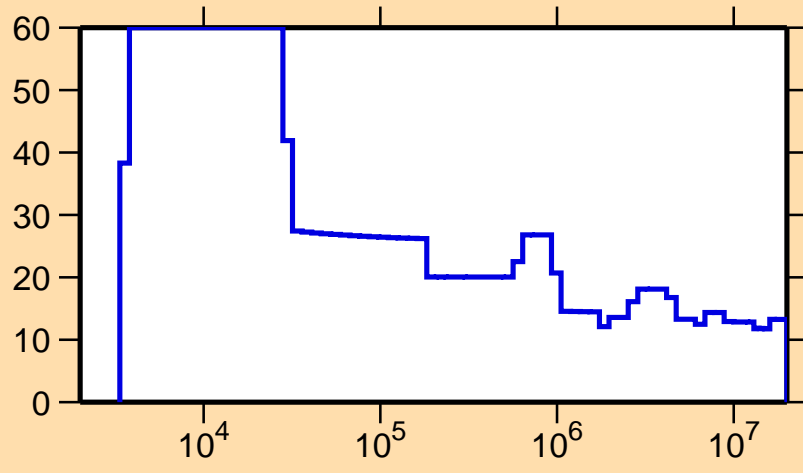
\Delta\sigma/\sigma vs. E for ^{190}\text{W}(n,\text{tot.})
