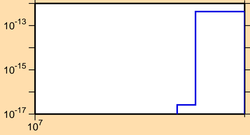
\sigma vs. E for ^{190}\text{W}(n,3n\alpha)
