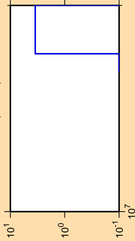
\Delta\sigma/\sigma vs. E for ^{190}\text{W}(n,3n\alpha)
