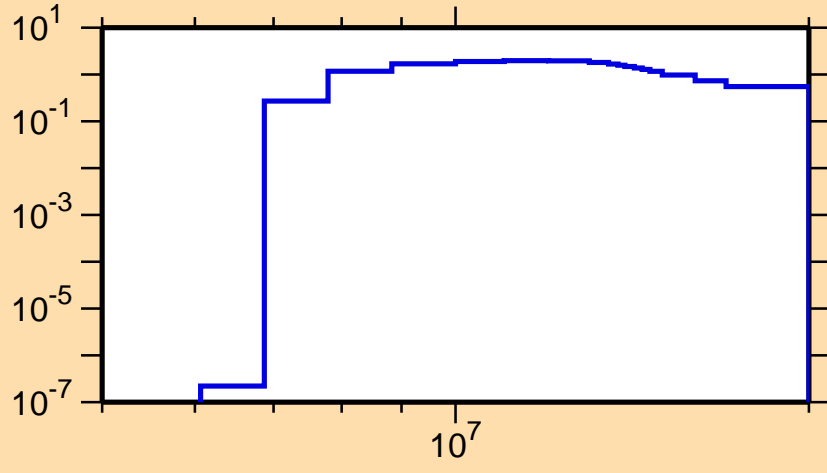
\sigma vs. E for ^{190}\text{W}(n,2n)
