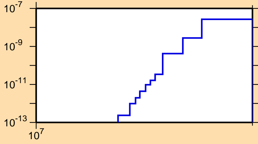
\sigma vs. E for ^{190}\text{W}(n,2n\alpha)
