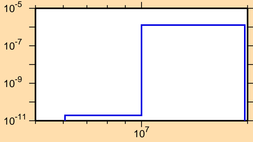
\sigma vs. E for ^{190}\text{W}(n,n\alpha)
