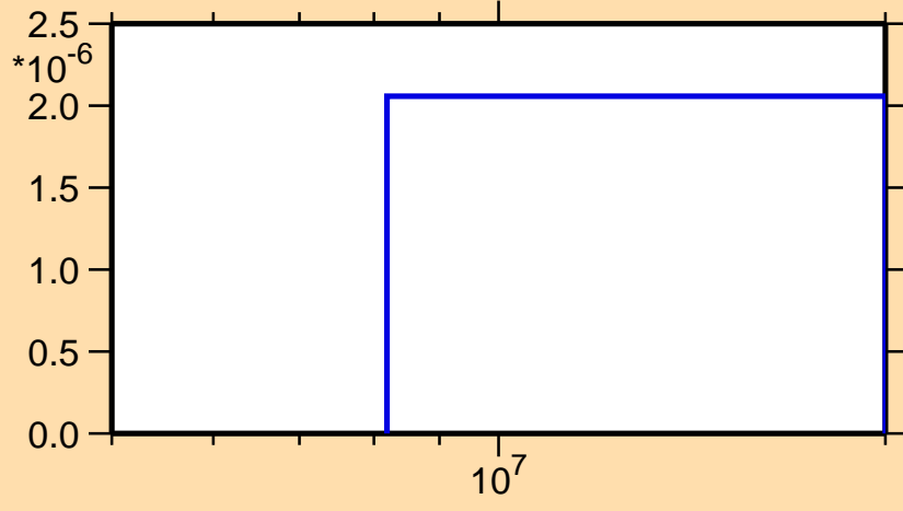
\sigma vs. E for ^{190}\text{W}(n,np)
