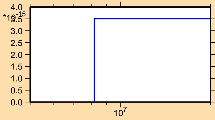
\sigma vs. E for ^{190}\text{W}(n,3n\alpha)
