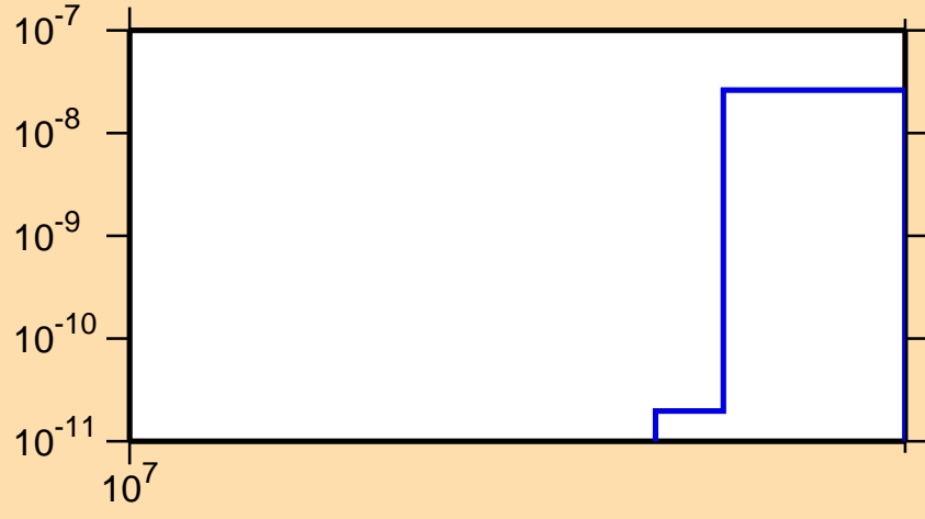
\sigma vs. E for ^{191}\text{W}(n,nt)
