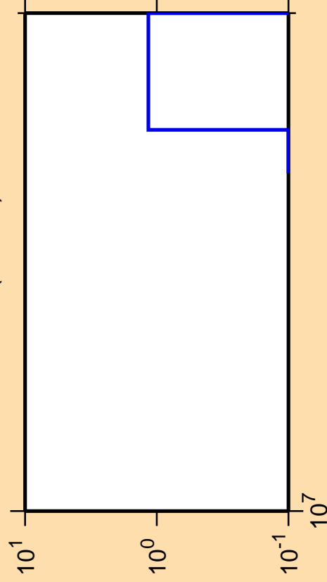
\Delta\sigma/\sigma vs. E for ^{191}\text{W}(n,3n\alpha)
