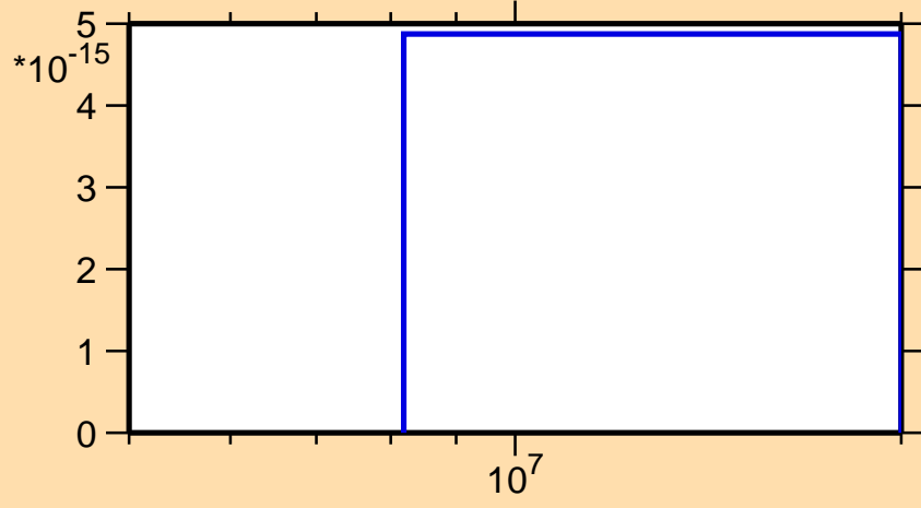
\sigma vs. E for ^{191}\text{W}(n,3n\alpha)
