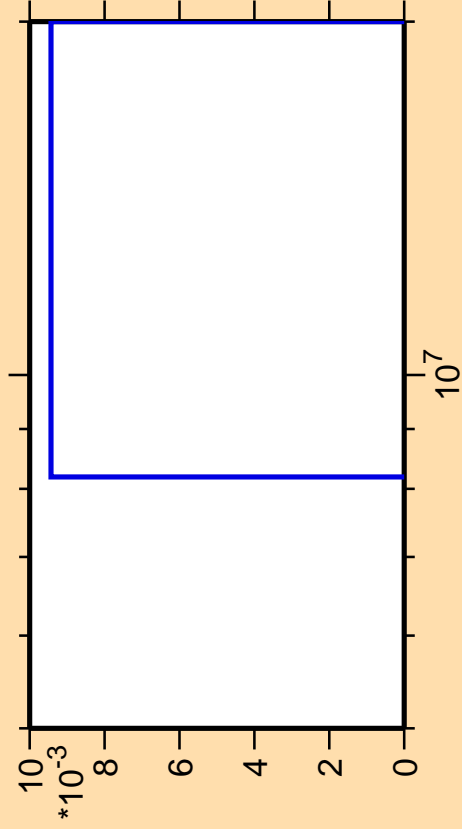
\Delta\sigma/\sigma vs. E for ^{191}\text{W}(n,3n\alpha)
