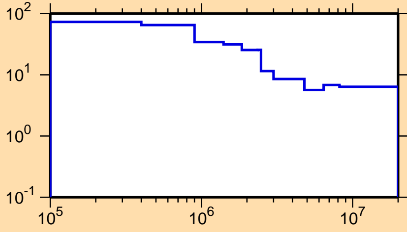
\Delta\sigma/\sigma vs. E for ^{191}\text{W}(n, nonel.)
