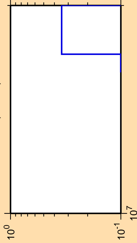
\Delta\sigma/\sigma vs. E for ^{192}\text{W}(n,3n\alpha)
