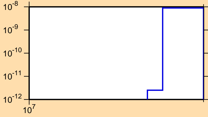
\sigma vs. E for ^{192}\text{W}(n,nt)
