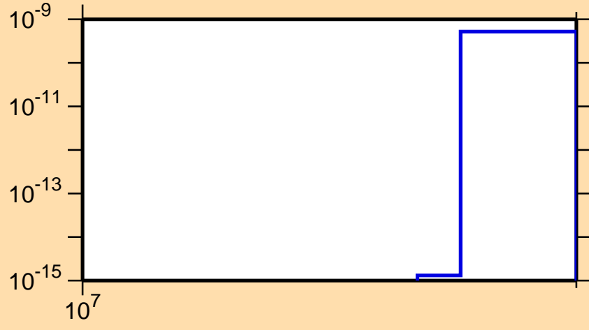
\sigma vs. E for ^{192}\text{W}(n,\text{nd})
