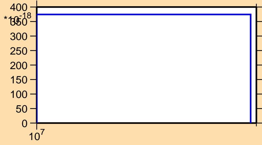
\sigma vs. E for ^{192}\text{W}(n,3n\alpha)
