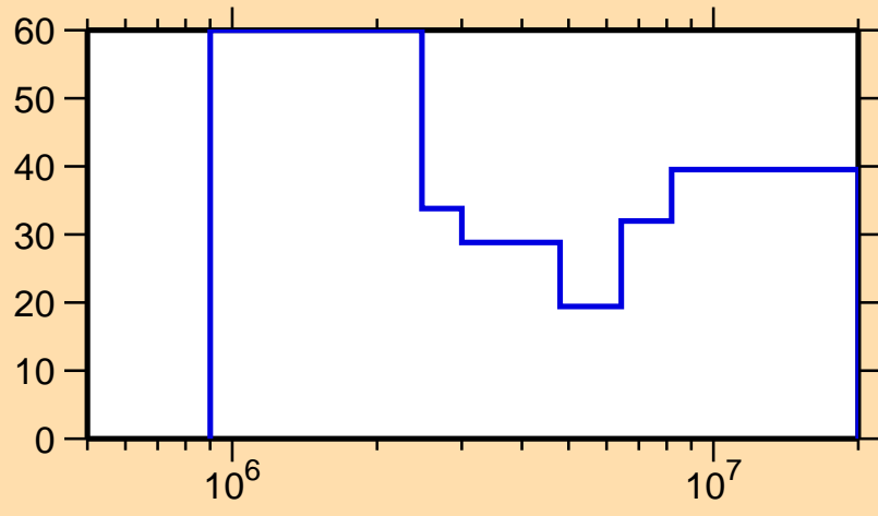
\Delta\sigma/\sigma vs. E for ^{192}\text{W}(n,n\text{cont.})
