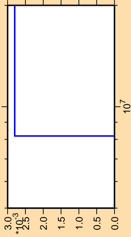
\Delta\sigma/\sigma vs. E for ^{192}\text{W}(n,3n\alpha)
