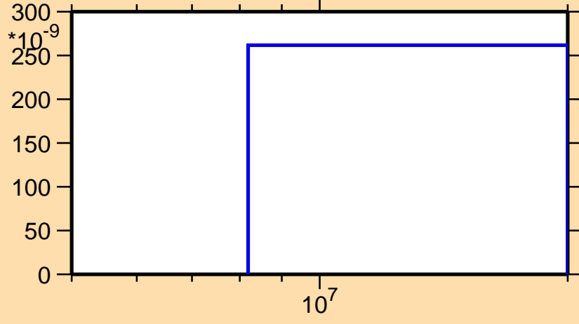
\sigma vs. E for ^{192}\text{W}(n,n\alpha)
