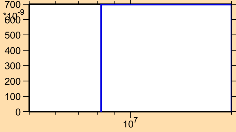
\sigma vs. E for ^{192}\text{W}(n,t)
