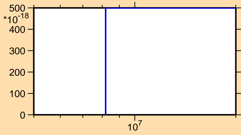
\sigma vs. E for ^{192}\text{W}(n,3n\alpha)
