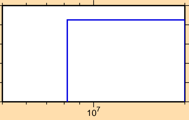
\sigma vs. E for ^{192}\text{W}(n,\text{nd})
