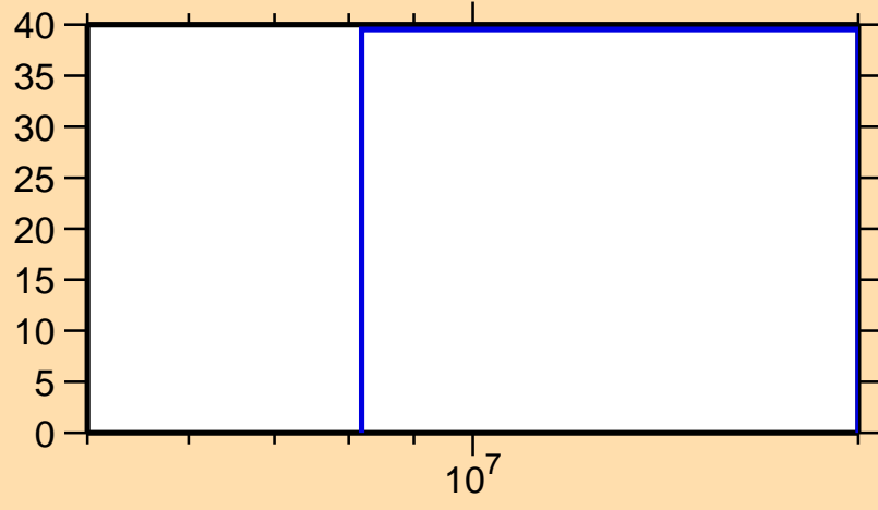
\Delta\sigma/\sigma vs. E for ^{192}\text{W}(n,ncont.)
