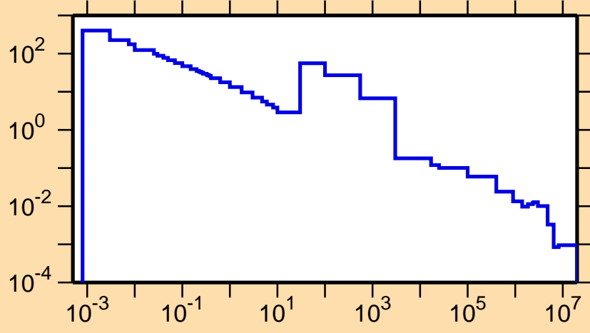
\sigma vs. E for ^{192}\text{W}(n,\gamma)
