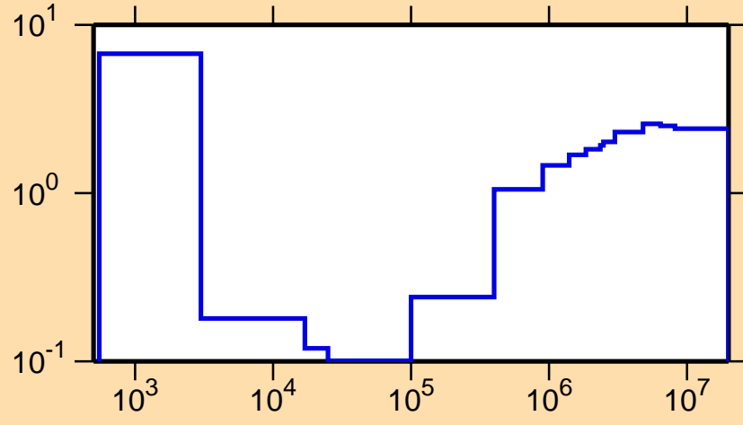
\sigma vs. E for ^{192}\text{W}(n,\text{nonel.})
