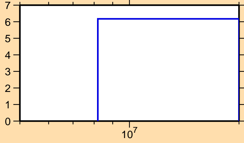
\Delta\sigma/\sigma vs. E for ^{192}\text{W}(n,\text{el.})
