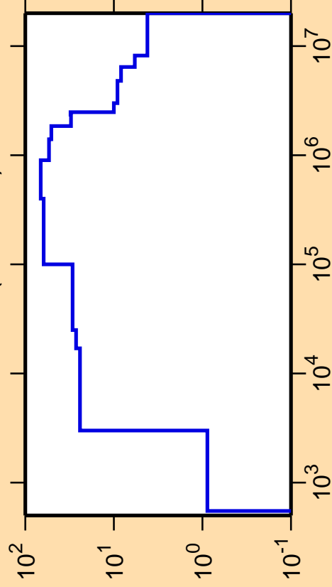
\Delta\sigma/\sigma vs. E for ^{192}\text{W}(n,\text{nonel.})
