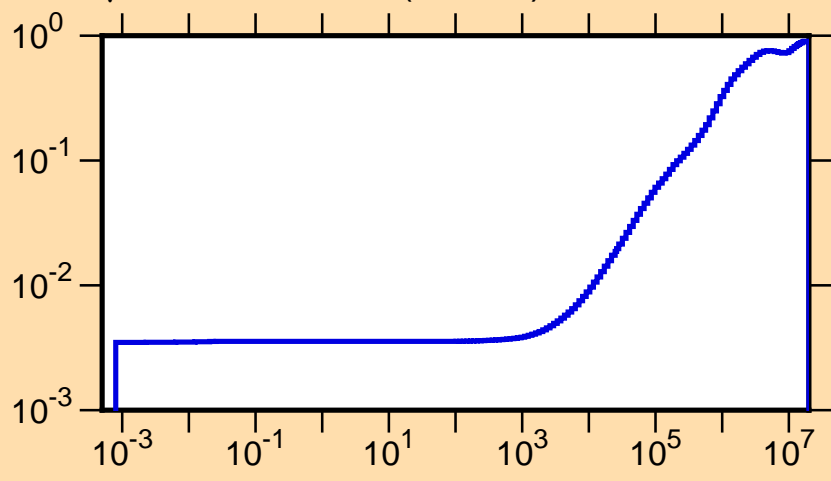
\mu vs. E for ^{193}\text{W}(\text{mt251})
