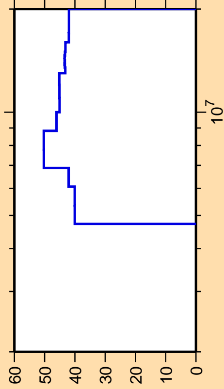
\Delta\sigma/\sigma vs. E for ^{193}\text{W}(n,n_1)
