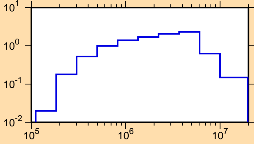
\sigma vs. E for ^{193}\text{W}(n,\text{inel.})
