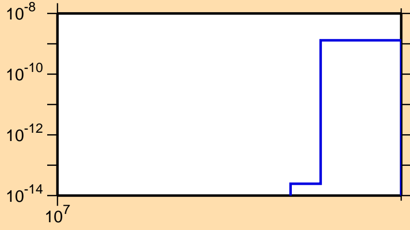
\sigma vs. E for ^{194}\text{W}(n,nt)
