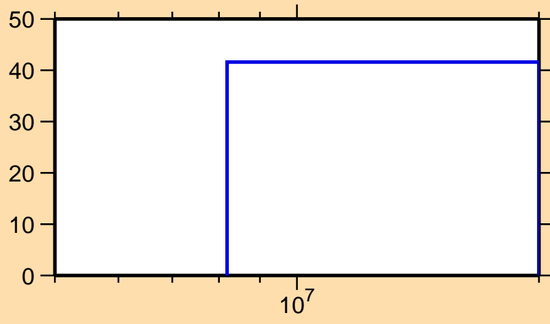
\Delta\sigma/\sigma vs. E for ^{194}\text{W}(n,p)
