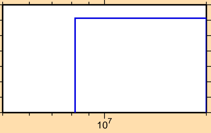
\sigma vs. E for ^{194}\text{W}(n,\text{nd})
