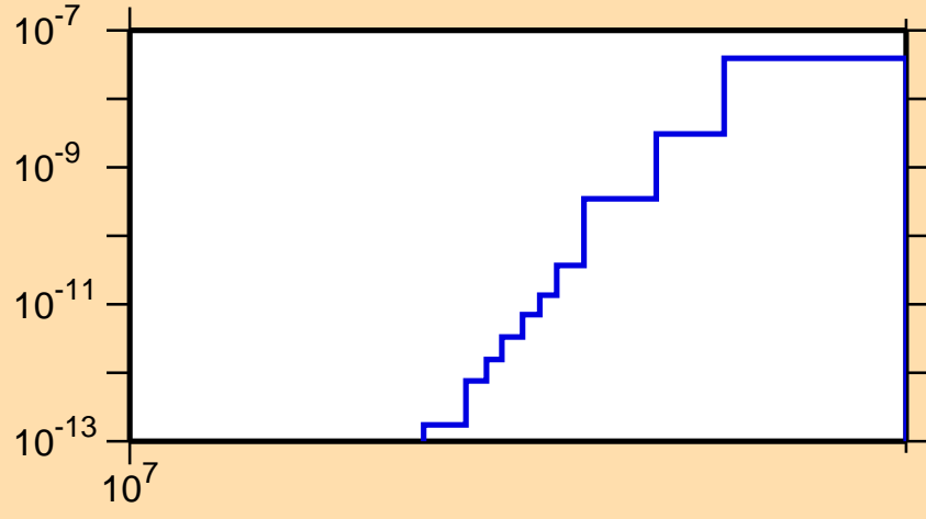
\sigma vs. E for ^{112}\text{Xe}(\text{mt } 34)
