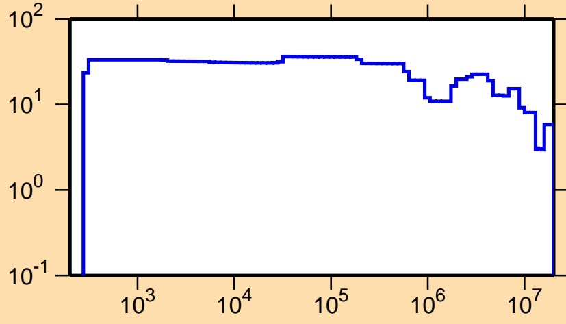
\Delta\sigma/\sigma vs. E for ^{112}\text{Xe}(n,el.)
