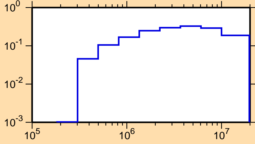
\sigma vs. E for ^{112}\text{Xe}(n,\text{inel.})
