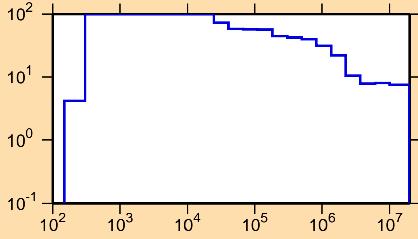
\Delta\sigma/\sigma vs. E for ^{112}\text{Xe}(n,\text{nonel.})
