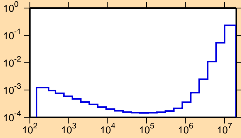
\sigma vs. E for ^{112}\text{Xe}(n,p\alpha)
