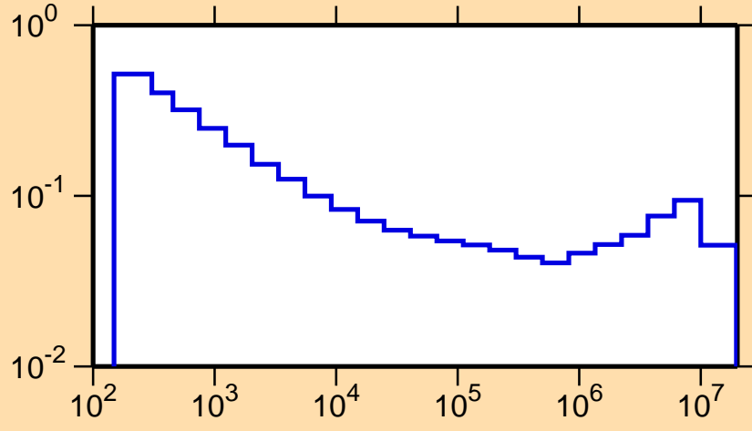
\sigma vs. E for ^{112}\text{Xe}(n,\alpha)
