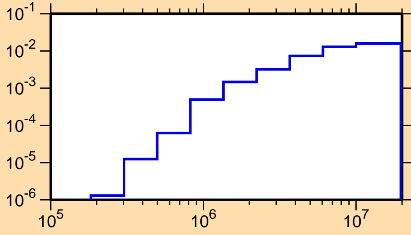
\sigma vs. E for ^{112}\text{Xe}(n,n\alpha)
