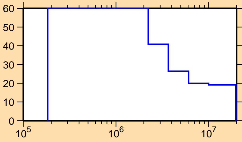
\Delta\sigma/\sigma vs. E for ^{112}\text{Xe}(n,n_1)
